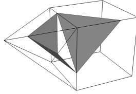
Figure 6. If the tessellation filling the gaps between hierarchy levels, which result from the use of dual grids, does not share complete boundary faces with rectilinear cells of the dual grid, cracks in an isosurface can result. This is a result of the fact, that the same curved contour on the boundary is represented at different detail, i.e., a single line on the rectilinear face and a polyline consisting of two line segments on the two triangular faces.
