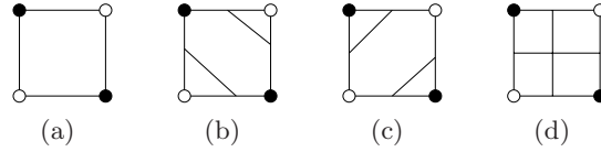
Figure 3. An ambiguous face configuration consists of vertices alternating between being inside and outside of the isosurface (a). Three different contour topologies on that face are possible: separating vertices outside the contour (b), separating vertices inside the contour (c), or separating all vertices (d) resulting in a non-manifold contour.
