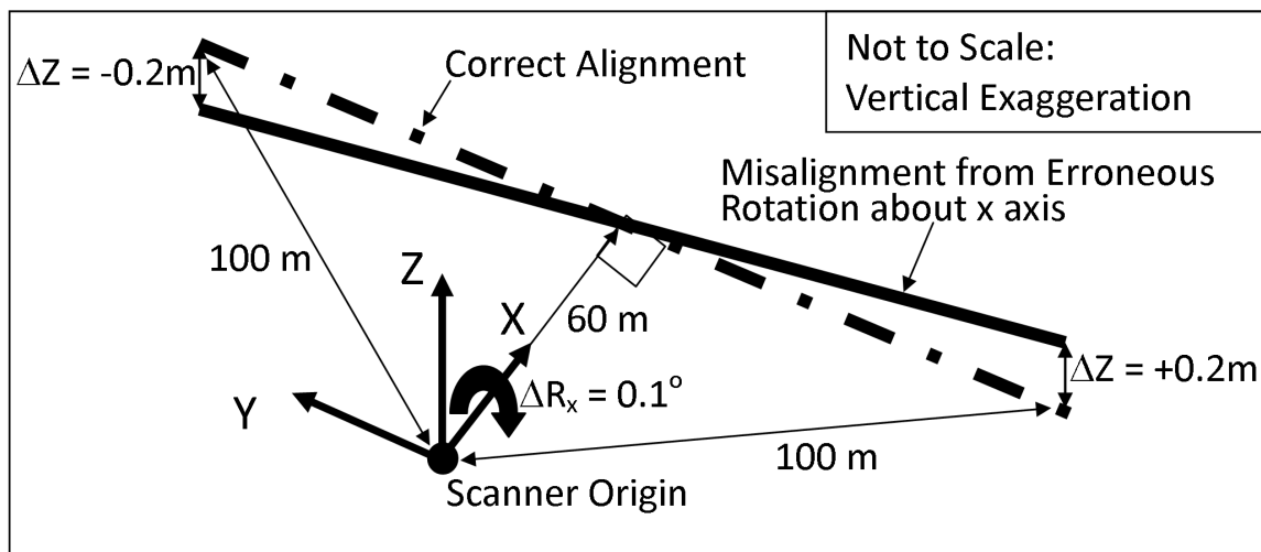
Figure 3-4. Misalignments from erroneous rotations about X or Y axis
