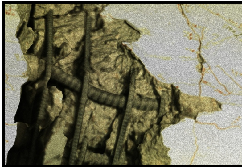
Figure 7-2. Close-up of surface mesh of failed structural specimen with overlaid texture map.
