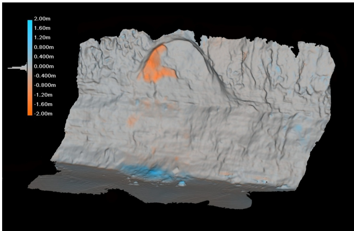
Figure 5-28. Surface change analysis for site TP6 comparing the post failure, June 18, 2008 survey to the pre-failure, April 28, 2008 survey
