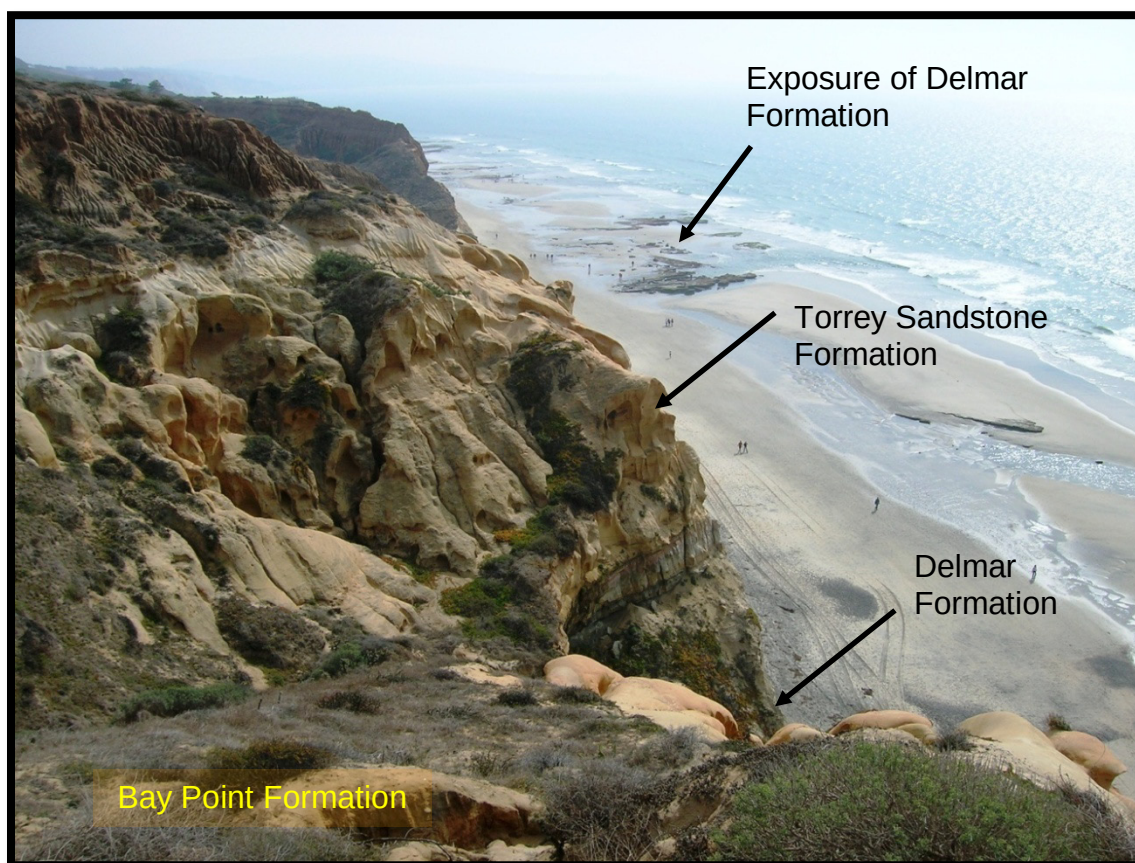
Figure 1-16. Geologic formations at Torrey Pines Reserve
