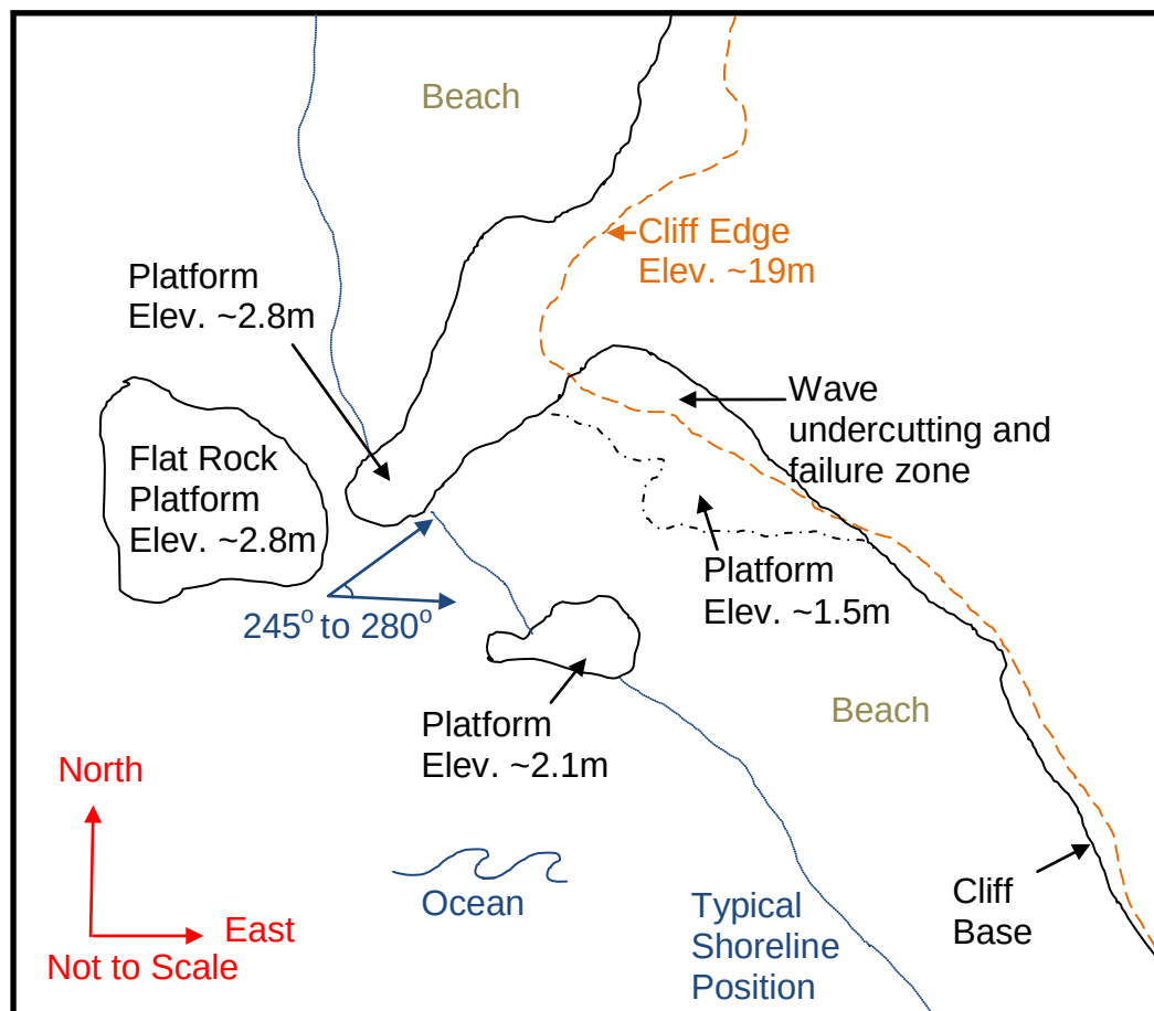
Figure 5-17. Plan view schematic showing cliff and platform geometry for Flat Rock, Torrey Pines Reserve. Note that an incoming peak wave direction of 245^\circ to 280^\circ measured clockwise from True North maximizes energy transfer to cliff at failure zone.
