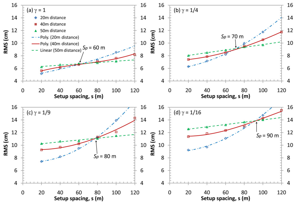
Figure 2-6. RMS uncertainty of adjacent scans at varying scan setup spacings for (a) full, (b) quarter, (c) ninth, and (d) sixteenth scanner sampling ratios ( \gamma ). Setup spacing pivot points ( s_p ) indicate where closer distances from the cliff produce higher RMS uncertainty.
