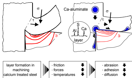
Figure 19: Layer formation in machining calcium treated steels [43].
