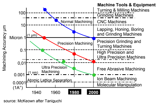
Figure 2: Taniguchi equivalent for cutting processes [modified by the authors].
