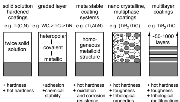
Figure 11: Structure of Coatings.
