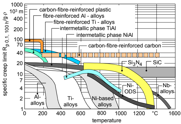
Figure 23: Materials for turbine manufacture [source: MTU].
