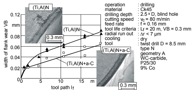
Figure 12: Wear performance of soft coated drills.
