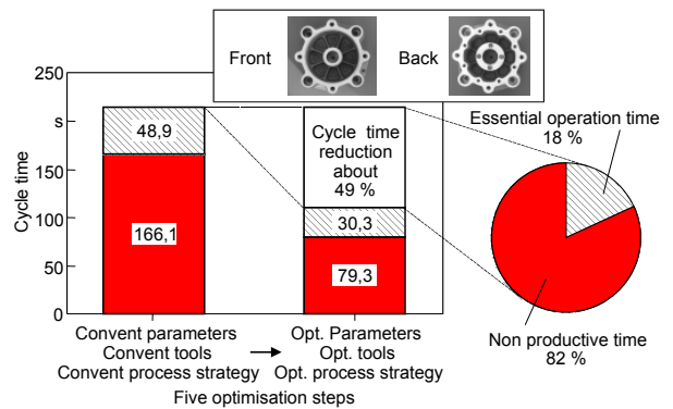
Figure 7: Reduction of the cycle time for machining a model workpiece [ISF].
