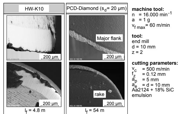
Figure 22: Tool wear in the end milling of particle reinforced wrought alloys [58].
