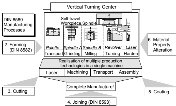
Figure 29: Integration of multiple processing technologies into vertical turning centers.
