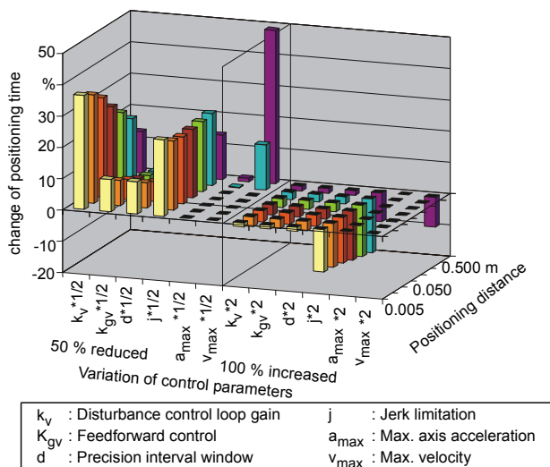
Figure 26: Positioning time of a machining center.
