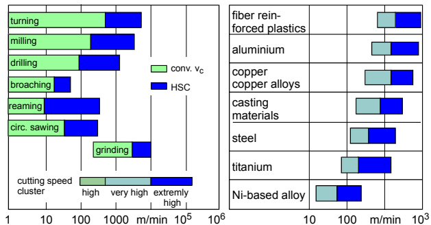
Figure 16: Achievable cutting speeds [34].
