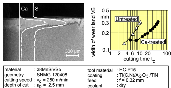
Figure 20: Influence of calcium treatment on tool life in turning with coated carbides [45].
