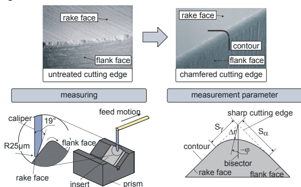
Figure 13: Characterisation of the cutting edge geometry.
