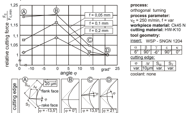
Figure 14: Cutting edge geometry and cutting forces.
