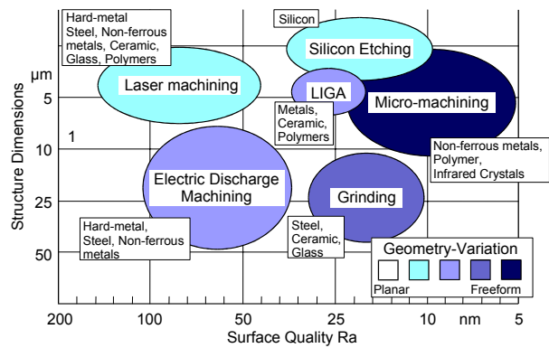
Figure 3: Micromachining relative to other machining processes [IPT-Aachen].
