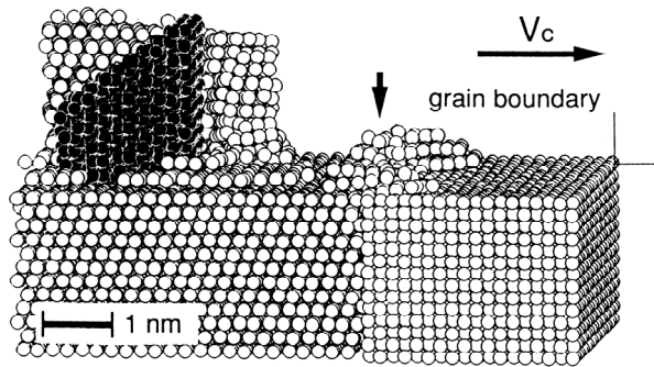
Figure 33: 2D and 3D molecular dynamics simulation of burr and chip formation in copper [141].
