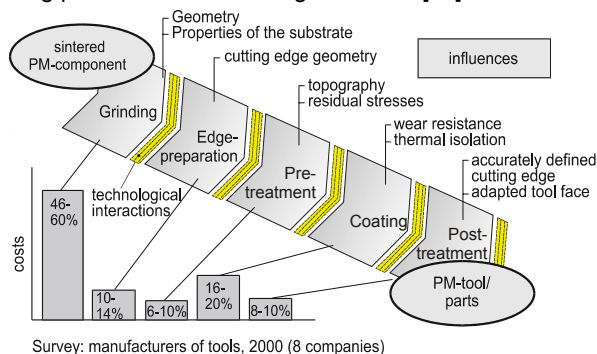
Figure 9: Manufacturing process of powder metallurgical tools.
