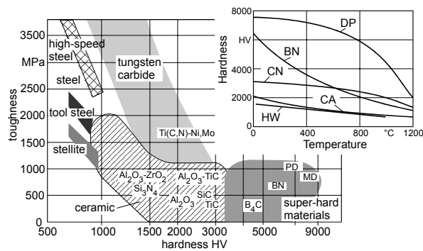
Figure 8: Toughness and hardness of cutting materials.
