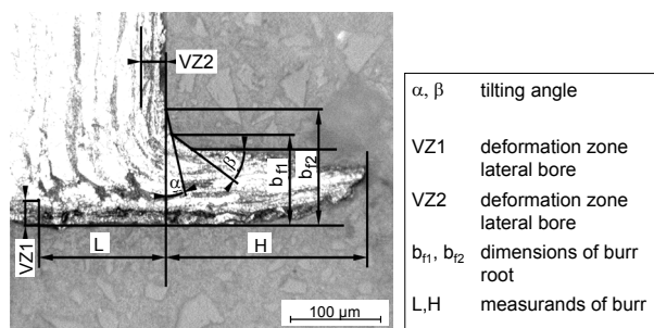
Figure 24: Typical burr and proposed measuring nomenclature [63].
