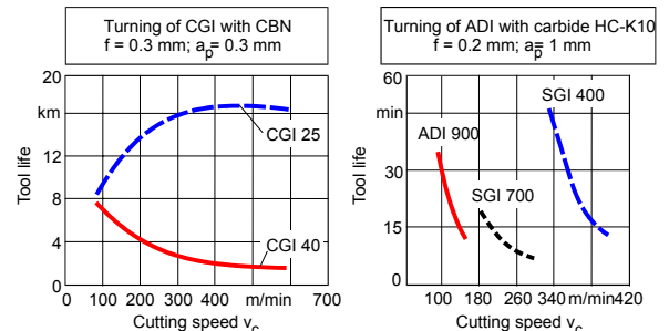
Figure 21: Demands on the cutting process in the turning of CGI and ADI [46, 47].
