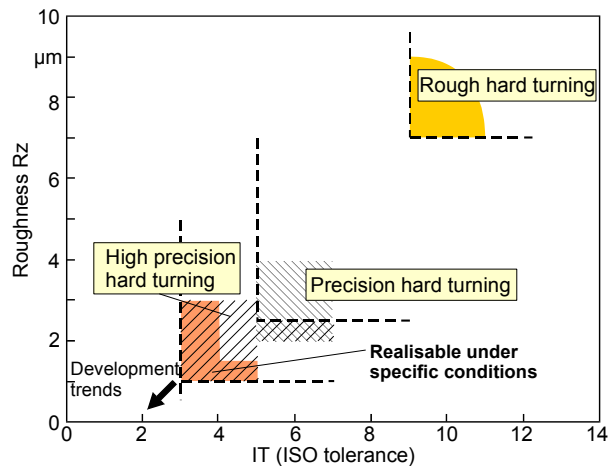
Figure 6: Roughness versus IT Tolerances for Hard Turning.
