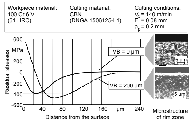
Figure 17: Residual stress and surface layer effects after hard turning [40].
