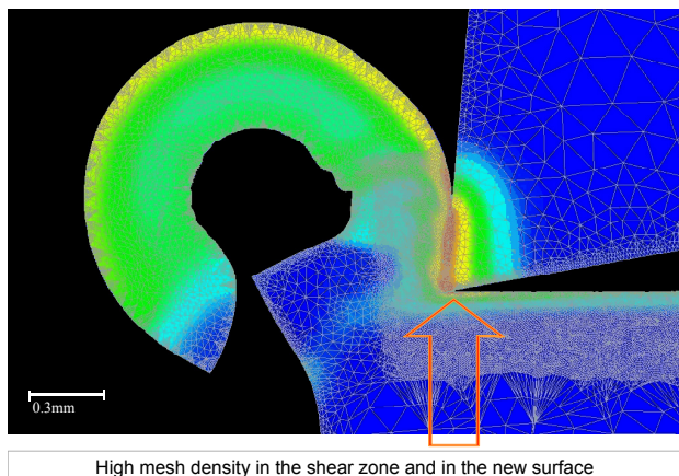
Figure 32: FEM simulation of burr formation in orthogonal cutting utilising different mesh densities [135].
