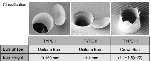
Figure 25: Three typical burrs in drilling stainless steel [64].
