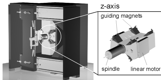
Figure 27: Machine tool with direct drives and magnetic guided z-axis.
