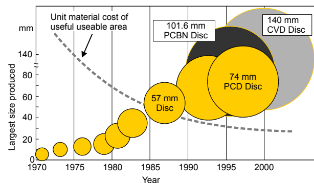
Figure 5: Cost reduction of superhard tool materials [source: Element 6].
