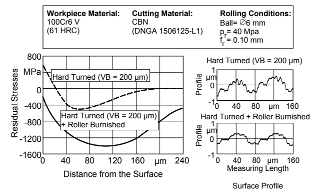
Figure 18: Surface layer effects due to roller burnishing [40].
