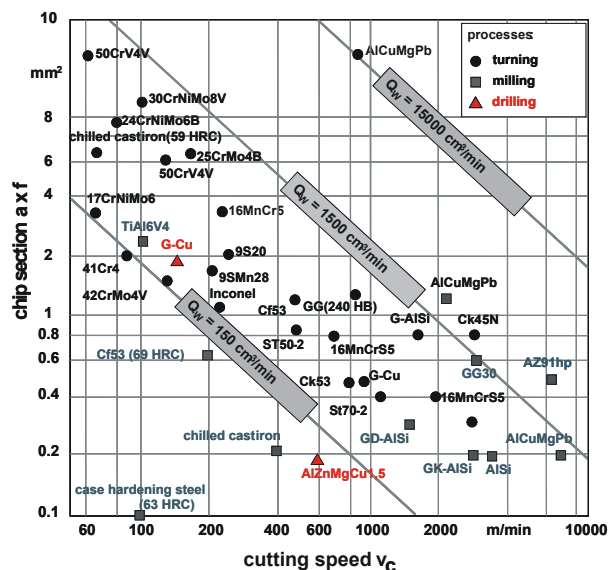
Figure 15: Material removal rates for a range of materials and cutting processes [33].
