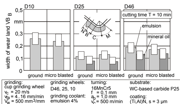
Figure 10: Influence of tool grinding on the cutting performance in turning.
