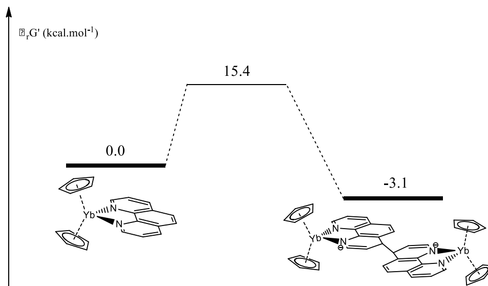
Figure 12. Reaction coordinate diagram for dimerization of \text{Cp}_2\text{Yb}(\text{phen}) .
