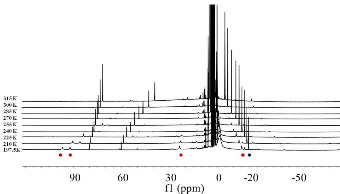
Figure 10. Stacked plot of ^1\text{H} NMR spectra in function of the temperature in THF. Red dots are the resonances used for integration of the asymmetric species and the blue dot is the resonance used for integration of the symmetrical species.
