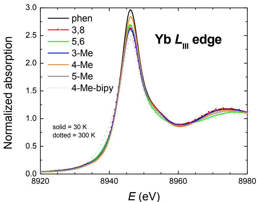
Figure 2. Yb L_{\text{III}} -edge XANES spectra for 1-dimer,3-7 at 30 K (solid) and at 300 K (dotted). Also shown are previous data 4 on \text{Cp}^*_2\text{Yb}(4\text{-Me-bipy}) ( n_f = 0.79 ) for comparison. The shoulder at 8939 eV below the main peak at 8946 eV is indicative of the Yb(II) contribution, which is clearly seen in the bipy adduct data. The strong overlap of all the measured phen adduct data emphasizes the overall similarity in f-orbital occupancy. The small shoulder for each of the phen adducts indicates these samples are close to trivalent Yb.
