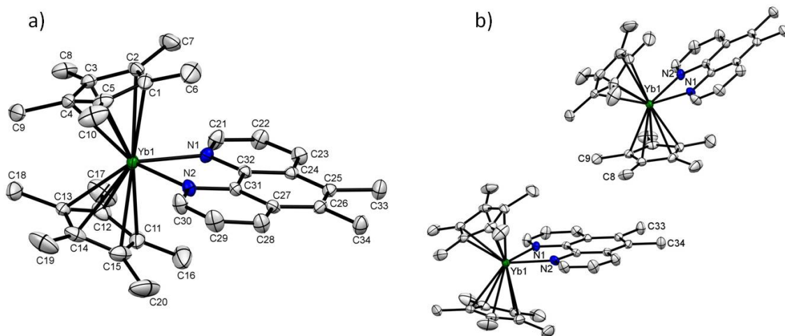
Figure 6a. ORTEP for crystallized \text{Cp}^*_2\text{Yb}(5,6\text{-Me}_2\text{phen}) ( 7, sublimed ) (thermal ellipsoids at 50% level). Ytterbium atom is in green, nitrogen atoms in blue and carbon atoms in grey. All non-hydrogen atoms are refined anisotropically and the hydrogen atoms are placed in calculated positions and refined isotropically. Hydrogen atoms have been omitted for clarity. 6b. A portion of the packing diagram showing two molecules in the unit cell, showing the shortest C...C contact distances are between C(8) and C(9) methyl groups on the \text{Cp}^* -ring and C(34) and C(35) methyl groups on the 5,6- \text{Me}_2\text{phen} ligand of 3.634 Å and 3.792 Å, respectively.
