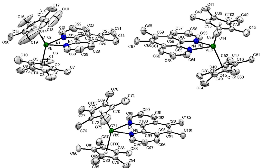
Figure 5: ORTEP for crystallized \text{Cp}^*_2\text{Yb}(5,6\text{-Me}_2\text{phen}) ( 7, crystallized ) (thermal ellipsoids at 50% level) showing the three independent molecules in the unit cell. Ytterbium atom is in green, nitrogen atoms in blue and carbon atoms in grey. All non-hydrogen atoms are refined anisotropically and the hydrogen atoms are placed in calculated positions but not refined. Hydrogen atoms have been omitted for clarity.
