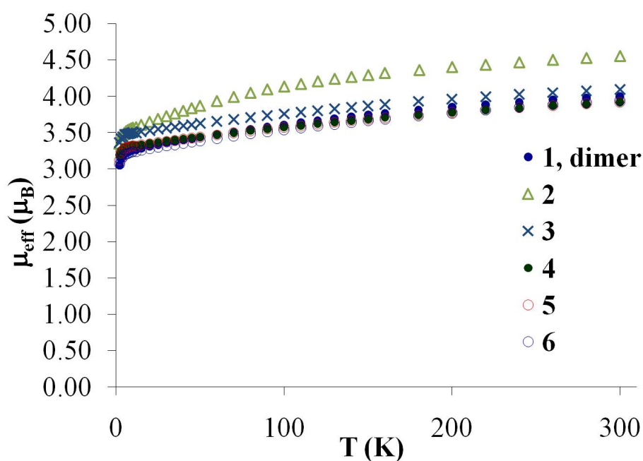
Figure 1a. Plot of the effective magnetic moment, \mu_{\text{eff}} , as a function of temperature for 1-6 in the 2-300 K temperature range. These adducts are obtained by crystallization.
