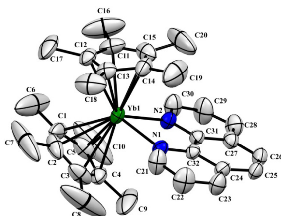
Figure 4: ORTEP for sublimed Cp* 2 Yb(phen) ( 1-monomer, sublimed ) (thermal ellipsoids at 50% level). Ytterbium atom is in green, nitrogen atoms in blue and carbon atoms in grey. All non-hydrogen atoms are refined anisotropically and the hydrogen atoms are placed in calculated positions but not refined. Hydrogen atoms have been omitted for clarity.
