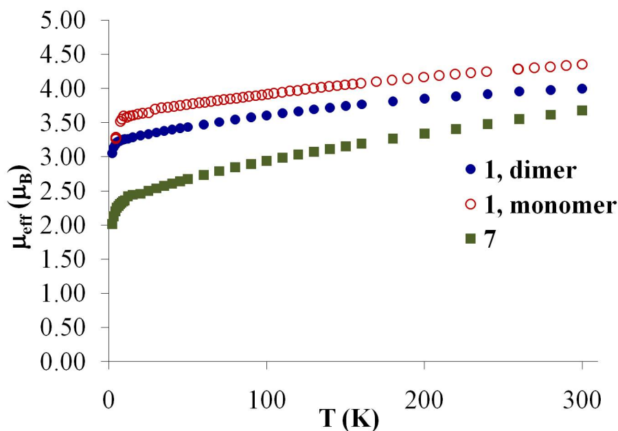
Figure 1b. Plot of the effective magnetic moment, \mu_{\text{eff}} , as a function of temperature for 1-monomer after sublimation (red unfilled dots), 1-dimer after crystallization (blue filled dots) and 7 after crystallization (green squares) in the 2-300 K temperature range.
