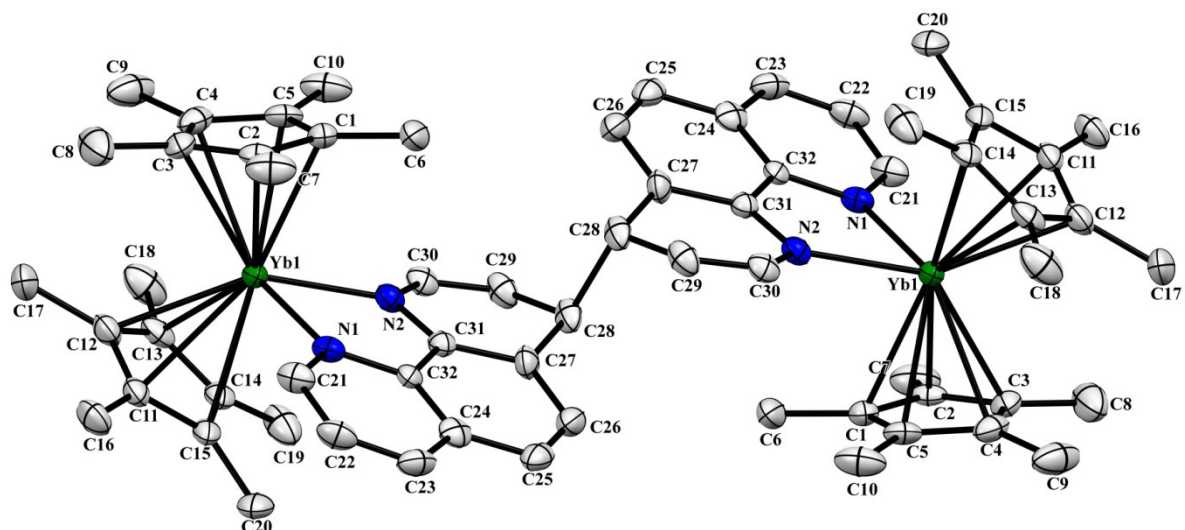
Figure 7: ORTEP for crystallized \text{Cp}^*_2\text{Yb}(\text{phen}) ( 1 ) (thermal ellipsoids at 50% level). All non-hydrogen atoms are refined anisotropically and the hydrogen atoms are placed in calculated positions but not refined. Hydrogen atoms have been omitted for clarity.
