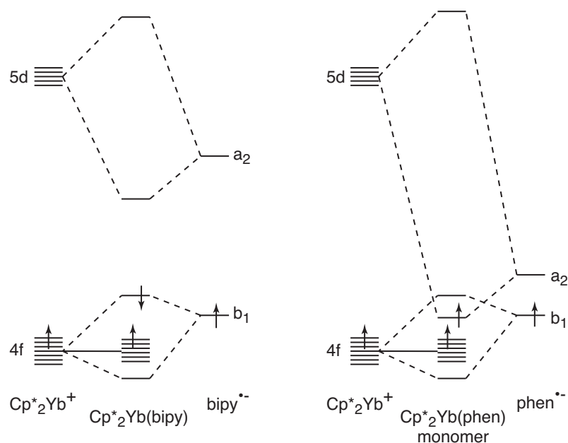
Figure 13. Qualitative MO diagram comparing bonding in Cp^*_2Yb(bipy) and Cp^*_2Yb(phen) monomer. Only the unpaired 4f electron is illustrated; the orbitals below those with arrows are filled. The direction of the arrows indicate the ground state: Cp^*_2Yb(bipy) has a singlet ground state while Cp^*_2Yb(phen) has a triplet ground state.
