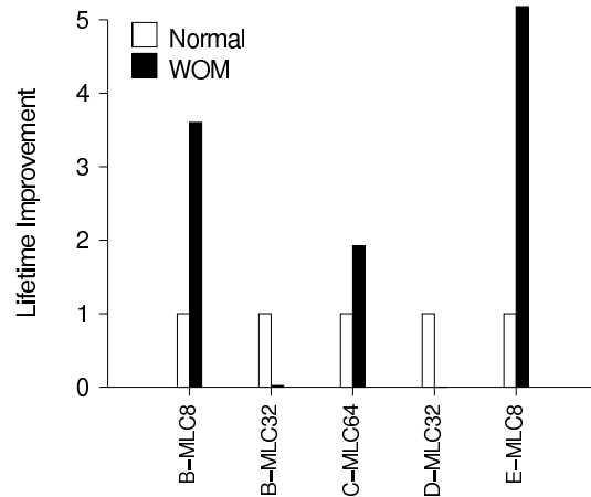
Figure 15: Effective device lifetime Measured in logical bytes written before the device reaches the fatal error rate, WOM codes allows up to 5.2 times longer lifetime.
