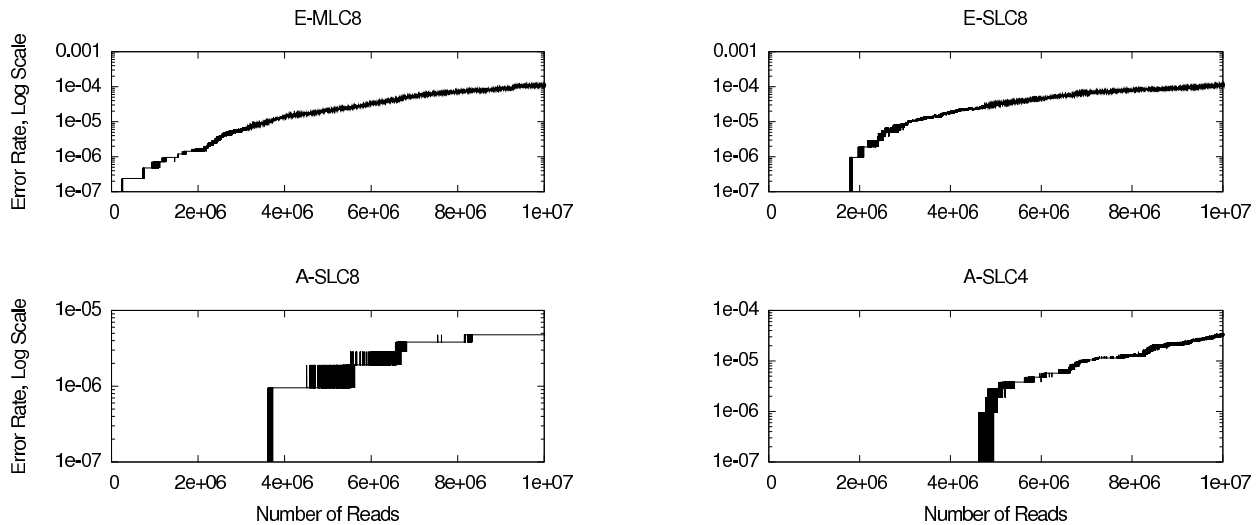
Figure 10: Read disturb up to 10 Million re-reads Repeatedly reading a page without refreshing the data causes a steadily increasing number of errors beginning at between 250 thousand and 4.8 million reads.
