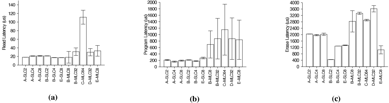
Figure 2: Flash operation latencies Average flash operation latency (excluding data transfer) for reads (a), programs (b), and erases (c) over ten program/erase cycles for 16 blocks on each chip. Error bars represent one standard deviation.
