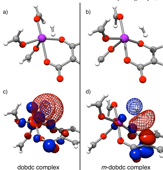
Figure 8. The calculated binding modes of H 2 in a) the dobdc complex and b) the m-dobdc complex, in both of which the Co 2+ is purple and the H 2 is above the Co 2+ . The corresponding COVPs are shown for c) the dobdc complex and d) the m-dobdc complex, with occupied and virtual orbitals shown as solid and mesh, respectively, at a 0.05 Å -3/2 isodensity.
