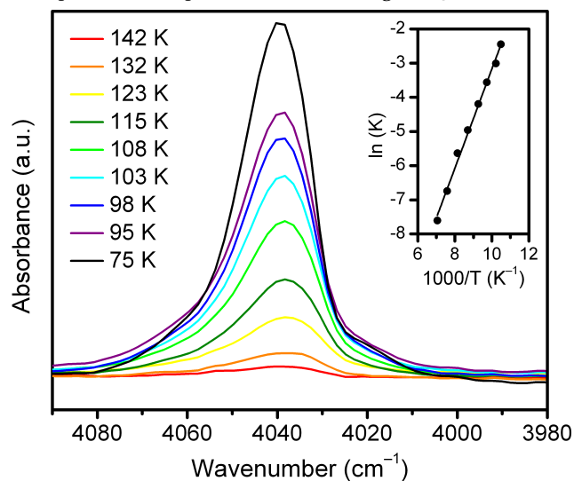
55 56 57 58 59 60 Figure 7. Variable temperature infrared spectra of \text{Co}_2(m\text{-dobdc}) . The inset shows the van't Hoff plot that is used to extract the enthalpy and entropy change in \text{H}_2 upon adsorption to the open metal site.
