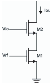
Figure 5.2: Double gate mixer.
