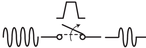
Figure 10.1: Conceptual Switching function
