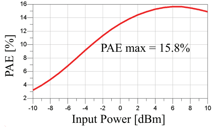
Figure 9.18: Simulated power added efficiency of the 90GHz power amplifier.
