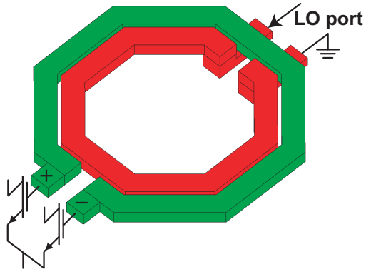
Figure 5.8: LO port balun structure.
