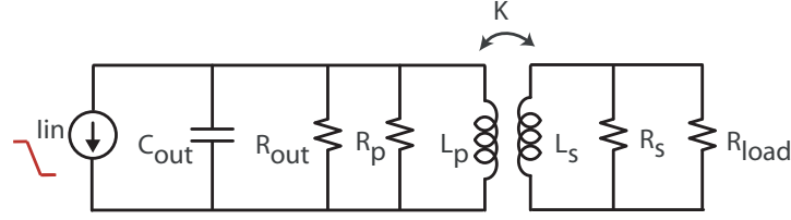
Figure 10.14: Simplified small signal model for the PA output stage
