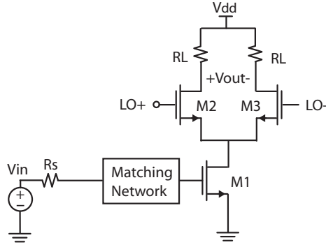
Figure 5.4: Single balanced active mixer.
