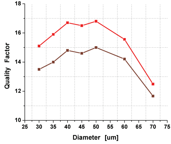
Figure 2.12: Quality factor versus internal diameter of the single-turn overlaid transformer with metal width= 6\mu m .
