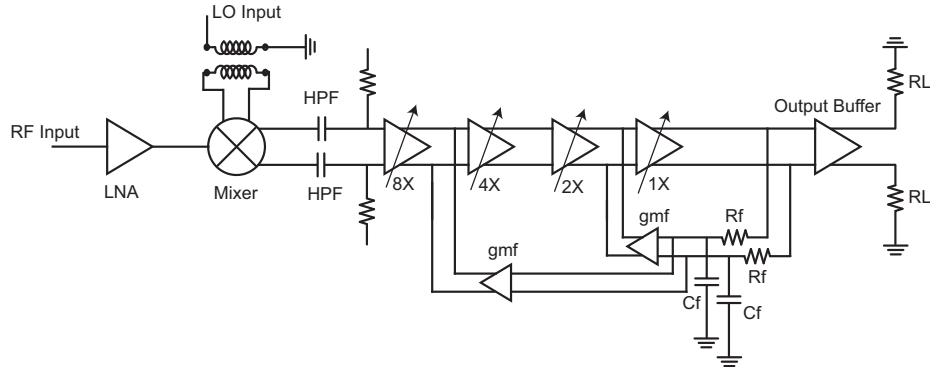
Figure 7.1: The core I or Q path implemented in this work.
