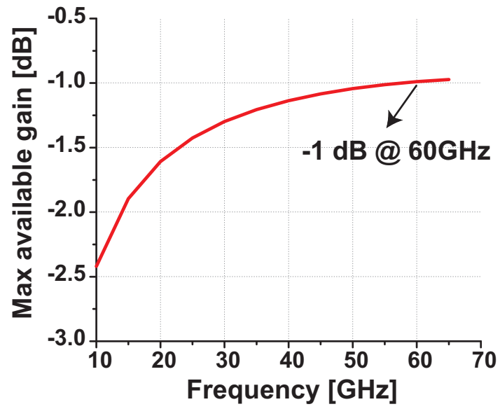
Figure 7.3: Measured balun maximum available gain.
