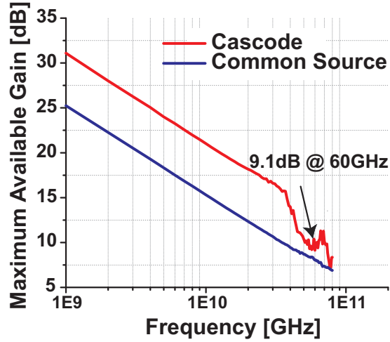
Figure 2.4: Measured NMOS common-source and cascode device performance: Maximum available gain.
