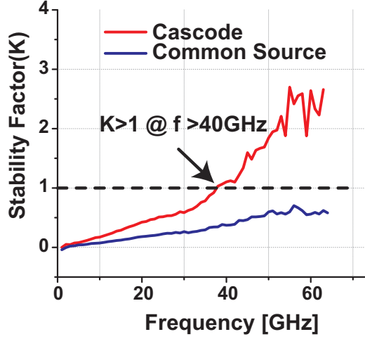
Figure 2.5: Measured NMOS common-source and cascode device performance: stability factor ( K ).
