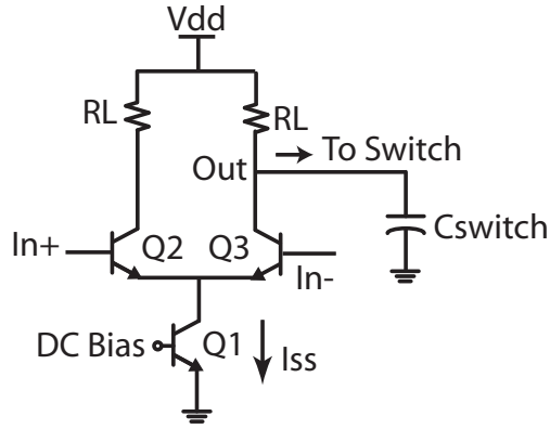
Figure 10.10: Schematic of the last stage of the switch driver.
