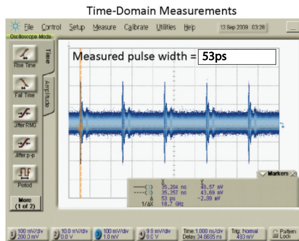
Figure 10.25: Time-domain pulse measurement in pulsed transmitter.
