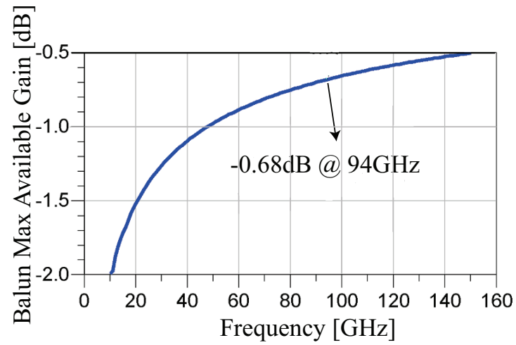
Figure 9.12: Simulated maximum available gain of power combining balun.
