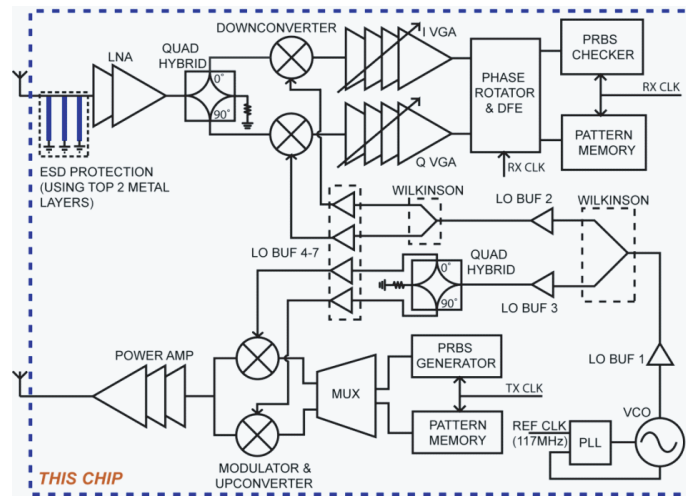
Figure 5.12: Block level schematic of the 60GHz transceiver chip [35].
