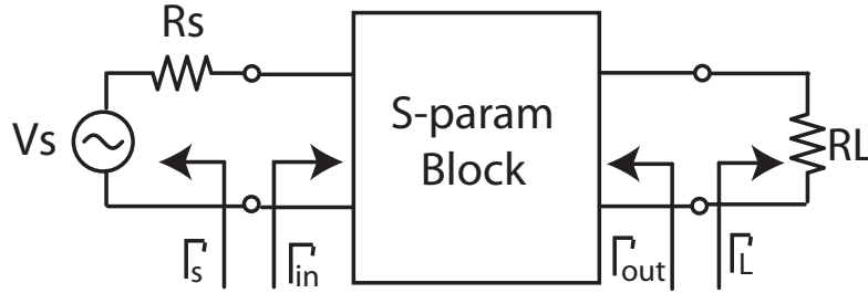
Figure 4.1: Two port S-parameter representation of active transistor.
