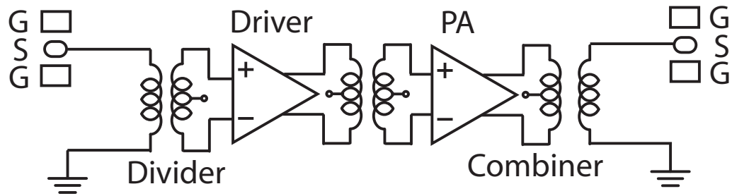
Figure 9.1: Block level schematic of the transformer coupled 90GHz power amplifier.
