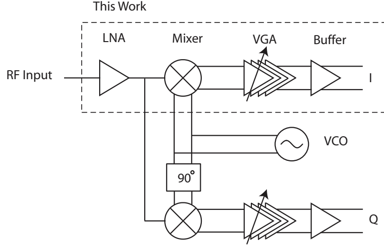
Figure 3.1: Block diagram of a direct-conversion receiver using I/Q paths.
