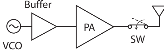
Figure 10.4: Switching after the power amplifier
