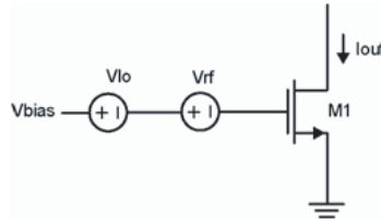
Figure 5.1: Single transistor active mixer.
