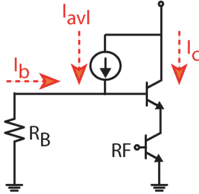
Figure 9.4: Avalanche current in bipolar transistor due to external impedance at the base junction.
