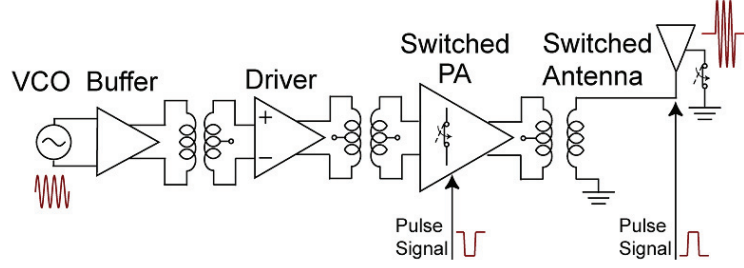
Figure 8.2: Sample of a simplified coherent pulsed transmitter [60].
