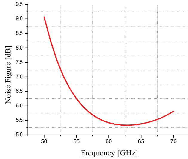
Figure 4.12: Simulated noise figure of the LNA.
