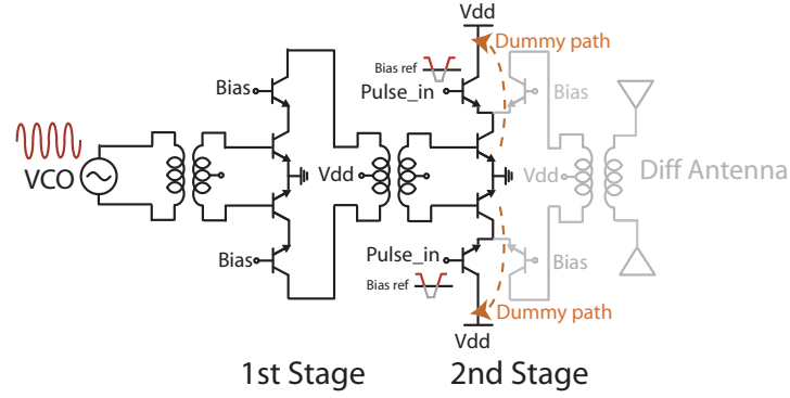
Figure 10.8: Switched PA in OFF mode.
