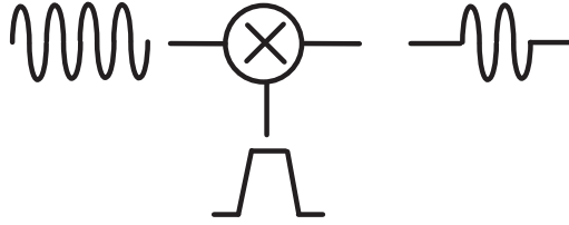
Figure 10.2: Conceptual Mixing functionality to generate carrier modulated pulsed signal
