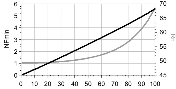
Figure 4.10: NF_{min} and R_n for a 40\mu cascode device. (Courtesy of Babak Heydari) [28]
