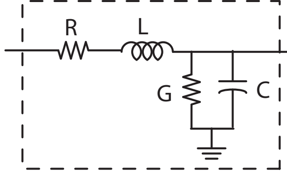
Figure 2.6: Small signal parameters of unit length transmission line.
