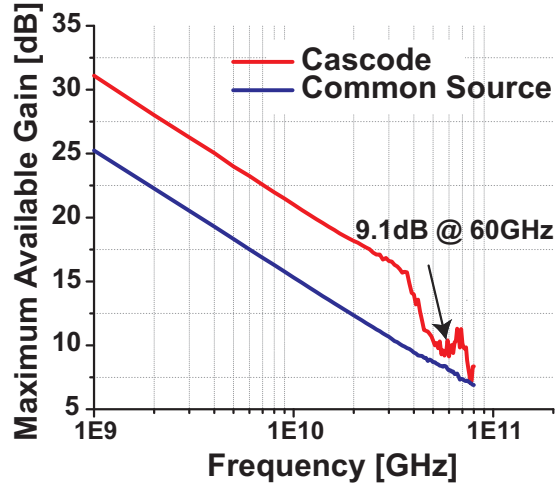
Figure 4.2: Maximum available gain of cascode and common source devices.
