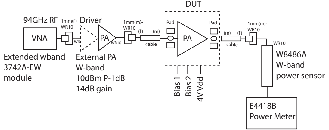
Figure 9.14: Measurement setup of W-band power amplifier.
