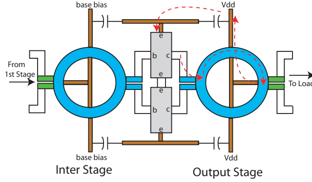
Figure 9.9: Common mode loop for interstage cascode transistors
