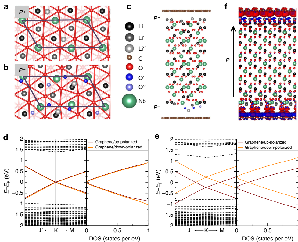
Figure 3 | Atomic and electronic structure of the graphene/ \text{LiNbO}_3 (0001) interface. Relaxed atomic surface structures of \text{LiNbO}_3 with graphene (not shown for clarity) adsorbed on the (a) up-polarized P^+ surface (with a 2 \times 1 nonstoichiometric reconstruction with an extra Li, denoted as \text{Li}' , per surface unit cell and an extra Li, denoted as \text{Li}'' , per every two surface unit cells) and (b) down-polarized P^- surface (with a 2 \times 1 nonstoichiometric reconstruction with an extra Li-O, denoted as \text{Li}' and \text{O}' , per surface unit cell and an extra Li-O, denoted as \text{Li}'' and \text{O}'' , per every two surface unit cells). The dark-purple line indicates the surface lattice periodicity. (c) Atomic structure of the 2 \times 1 surface reconstructed slab with graphene adsorbed on both terminations, reconstructed adatoms and two trilayers ( \text{LiO}_3 -Nb) near each interface are allowed to relax while the rest of the film, in this case, is fixed to the P(298 \text{ K}) = 0.875 P_0 atomic positions. Colour-coded labels indicate the ions that substantially passivate the polarization surface charge in the surface reconstruction. (d) Electronic band structure of graphene on both up- and down-polarized ferroelectric surfaces demonstrating that graphene is intrinsic for both interfaces in a relaxed slab with internal bulk ferroelectric polarization fixed to P(473 \text{ K}) = 0.8 P_0 , where the surface charge is essentially fully passivated by the 2 \times 1 reconstruction. (e) Induced charge redistribution as the graphene/ferroelectric interfaces are formed, where red indicates the gain of electrons (up-polarized, top surface) and blue the gain of holes (down-polarized, bottom surface), for the hybrid structure shown in b. The isovalue used to plot the charge density differential is 0.002 e \text{ \AA}^{-3} . (f) Electronic band structure of graphene on both up- and down-polarized ferroelectric surfaces demonstrating that graphene becomes n -doped and p -doped, respectively, passivating the extra surface charge that emerges in the 2 \times 1 reconstructed surfaces as temperature is reduced from 473 to 298 K and the ferroelectric polarization increases from P(473 \text{ K}) = 0.8 P_0 to P(298 \text{ K}) = 0.875 P_0 .
