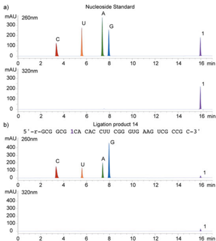
Fig. 4. HPLC profile of enzymatic digestion reactions. (a) A mixture of nucleosides used as a standard and (b) digestion results of ligation product 14 . Digestion of 1–2 nmol of transcript was carried out using S1 nuclease for 2 h at 37 °C and followed by dephosphorylation with alkaline phosphatase for 2 h at 37 °C. The ribonucleoside mixture obtained was analyzed by reverse-phase analytical HPLC with Agilent column eclipse XDB-C18 (5 \mu m, 4.6 \times 150mm). Mobile phase: 0–5% acetonitrile (0.1% formic acid) in water (0.1% formic acid) over 10 min and then increase 5–35% acetonitrile (0.1% formic acid) in water (0.1% formic acid) 10–17 min; flow rate 1 mL/min.
