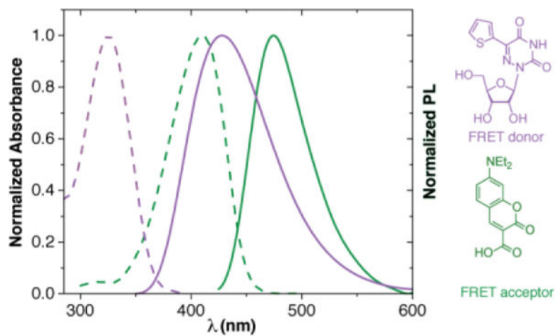
Fig. 7. Normalized absorption (---) and emission (—) spectra of 5-thiophene-6-azauridine in purple ( 1 ; FRET donor) and coumarin in green (FRET acceptor).
