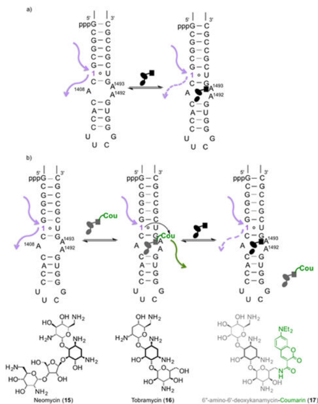
Fig. 5. (a) Binding of aminoglycosides to a fluorescently modified A-site hairpin 14 . (b) Binding and displacement events of A-site bound coumarin-aminoglycoside with unlabelled RNA binders (where 6-aza modified uridine 1 is a FRET donor and coumarin is a FRET acceptor).
