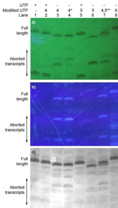
Fig. 3. Transcription reactions were carried out with T7 promoter and template A in the presence of natural NTPs and UTP or modified UTPs 4 , 5 , 6 . Lane 1: control reaction with all natural NTPs; lane 2: competition reaction in the presence of equimolar concentration of UTP and 4 , lane 3: reaction in the presence of 4 , lane 4: reaction in presence of 4 (*5mM instead of 1mM, as for all other reactions), lane 5: reaction in the presence of equimolar concentration of UTP and 5 , lane 6: reaction in the presence of 5 , lane 7**: reaction in the presence of equimolar concentration of 4 and 5 , lane 8: reaction in the presence of 6 . The reaction was resolved by gel electrophoresis on a denaturing 20% polyacrylamide gel; under UV light at a) 254 nm (on TLC plate); b) 365 nm; c) black and white picture after Stains-All was used to visualize the oligonucleotides.
