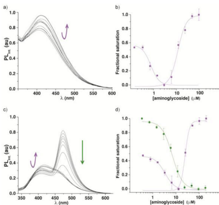
Fig. 6. Fluorescence titrations of the A-site construct 14 with neomycin ( 15 ). (a) Representative emission spectra for titrations of A-site hairpin 14 with neomycin. (b) Curve fit for the titrations of A-site hairpin 14 with neomycin ( 15 ) with respective values EC_{50} 0.9 \pm 0.2 \times 10^{-3} mM and 2 \pm 1 \times 10^{-2} mM (fractional saturation vs. antibiotic concentration). (c) Representative emission spectra for displacement studies: titrations of A-site hairpin 14 with neomycin ( 15 ). (d) Curve fit for the displacement studies: titrations of A-site hairpin 14 with neomycin with respective values EC_{50} 3.0 \pm 0.1 \times 10^{-3} mM and 3 \pm 1 \times 10^{-2} mM [fractional saturation vs antibiotic concentration; 1 , FRET donor (purple), 6''-amino-6''-deoxykanamycin-coumarin conjugate, FRET acceptor (green)]. Each event was fitted separately (see SI for details).
