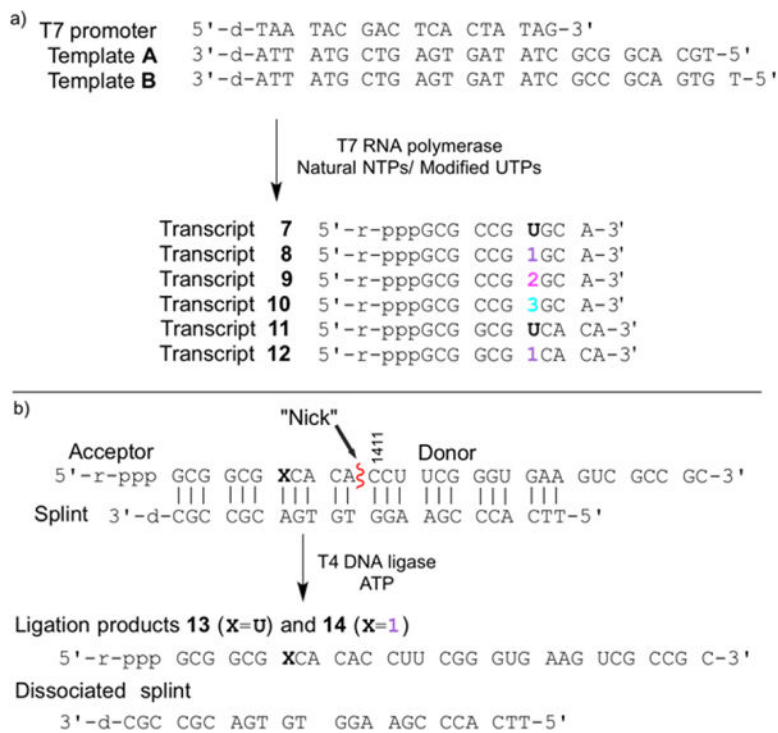
Fig. 2. (a) Transcription reaction with T7 promoter and template A in the presence of natural NTPs and UTP or modified UTPs 4–6 ; resulting in transcripts 7–10 respectively. Transcription reaction with T7 promoter and template B in the presence of natural NTPs and UTP or modified 4 , resulting in transcripts 11, 12 respectively. (b) Ligation reaction with T4 DNA ligase, modified acceptor, donor and splint.
