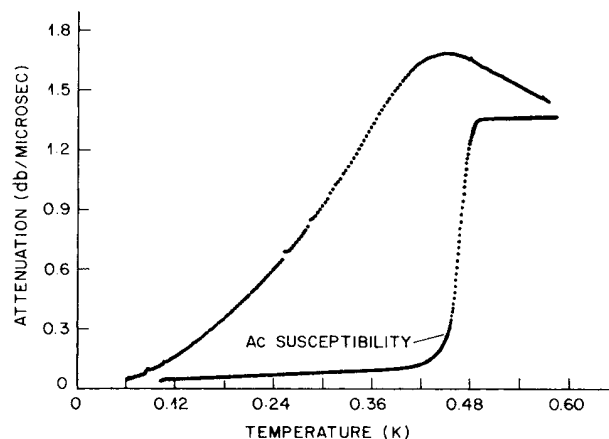
FIG. 1. The measured ultrasonic attenuation (at 507.9 MHz) and ac susceptibility for \text{UPt}_3 as functions of temperature. The velocity of sound is 3.9 \times 10^5 cm/sec.
