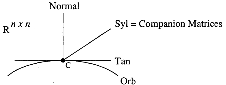
Figure 1 Matrix space near a companion matrix
