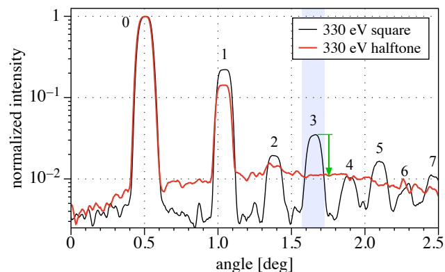
Fig. 5. Measurement of the same two gratings as Fig. 4, illuminated at 330 eV. The blue stripe identifies the first-order position for 110 eV and shows how the third order of 330 eV can overlap.
