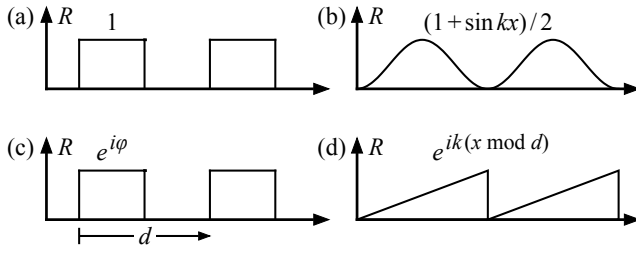
Fig. 1. Idealized grating models: (a) binary amplitude, (b) sinusoidal amplitude, (c) binary phase, (c) blazed.
