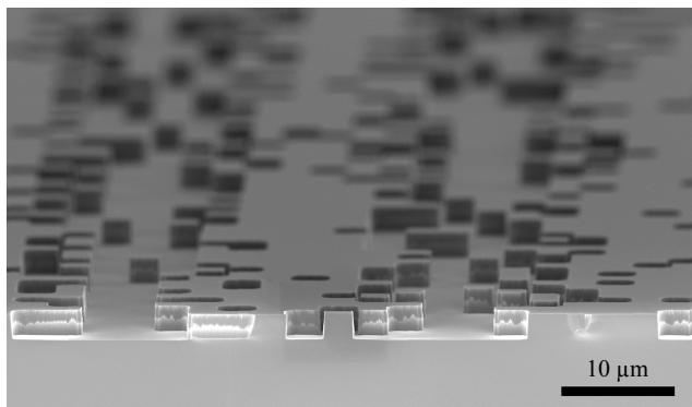
Fig. 3. Scanning electron microscope micrograph of the half-tone grating with 30 \mu\text{m} pitch, 3 \mu\text{m} pixels, and a 2.5 \mu\text{m} approximate etch depth. The wafer was cleaved to provide this inspection.
