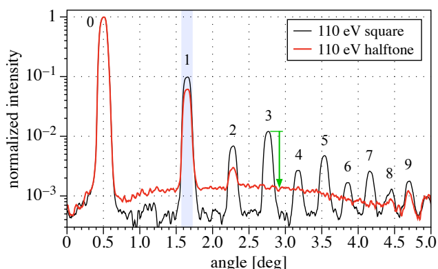
Fig. 4. Binary amplitude grating diffraction measurements, comparing square-wave (black) and sinusoidal half-tone (red). Gratings are illuminated with 110 eV soft X-ray light at 0.5^\circ incidence. The positions of the various grating orders are labeled, with the blue stripe identifying the first-order.
