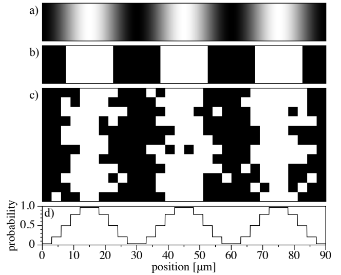
Fig. 2. Three reflective grating designs with pitch d = 30 \mu\text{m} . (a) Sinusoidal amplitude pattern ranging from 0 to 1. (b) Equal line-space binary amplitude pattern. (c) Detail of the pixelated halftone with a 3 \mu\text{m} pixel pitch, based on a discretized sinusoidal probability function derived from (a). Plot (d) shows the vertically integrated and normalized halftone pattern's amplitude, column by column. As shown, the gratings would be illuminated in the horizontal direction.
