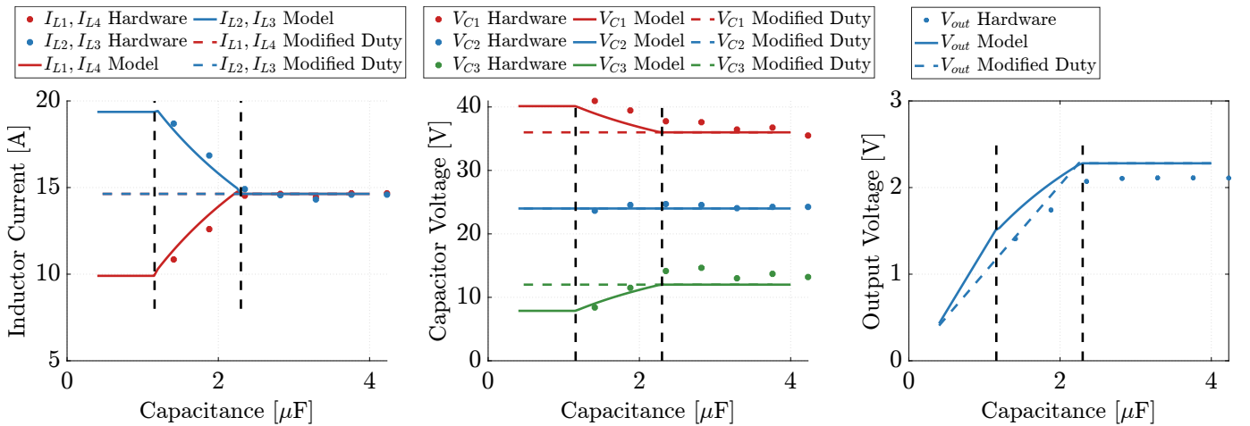
Fig. 5: Average inductor currents (left), midrange flying capacitor voltages (middle), and output voltage (right) measured on hardware, predicted by the steady-state DCVM model of section II-B, or for the modified duty cycle scheme of section II-C for several values of the flying capacitance.
