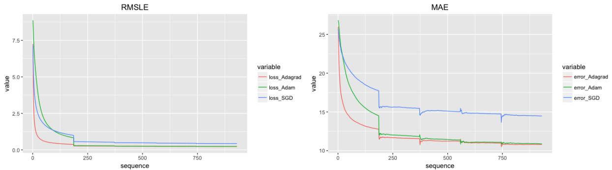
Figure 16: The training performance of 3 models over all batches over 5 epoches
