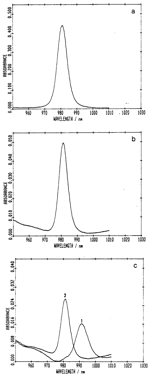
Figure 6. Near-IR absorption spectra of Np supernatant solutions at steady-state formed in J-13 groundwater at 90°C. (a) pH 5.9, (b) pH 7.2, (c) pH 8.4: (2) solution (1) acidified with \text{HClO}_4 to pH 0.
