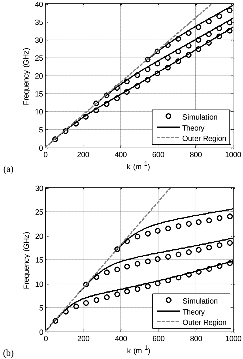
Figure 4.10: Frequency vs. wavenumber plot for a checkerboard guide. The tensor impedance is Z_{trans} = j133\Omega and (a) Z_{prop} = j399\Omega , (b) Z_{prop} = j1330\Omega . The simulated points are shown as circles. The theory line is the response as predicted from the ray-optics method. The line labeled Outer Region represents the dispersion relationship of a surface wave on a uniform surface with Z_2 = j133\Omega . This is the (isotropic) impedance of the region outside the guide.
