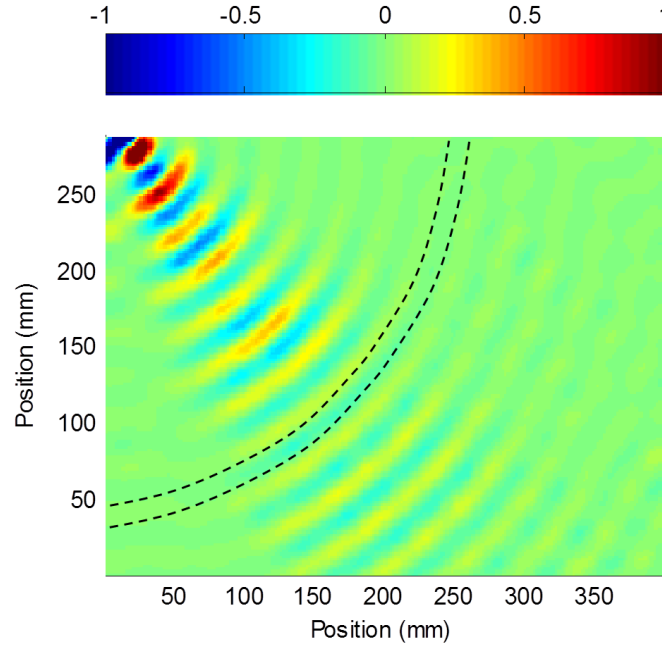
Figure 4.32: Measured field of orthogonally incident mode. The plot shows normalized vertical electric field at 12 GHz.
