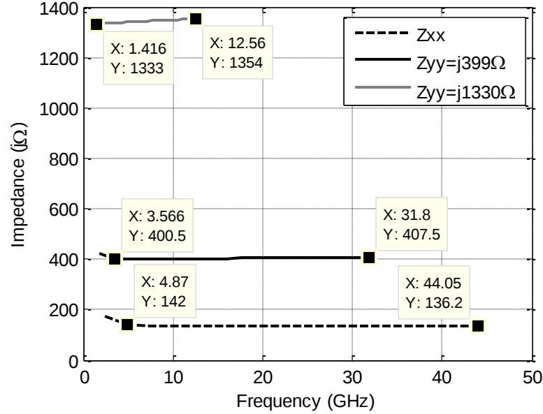
Figure 4.6: Impedance vs. frequency. The waves propagate in the X- and Y-directions. Two different Y (propagating) direction impedances were tested, Z_{yy}=j399\Omega and Z_{yy}=j1330\Omega . All other parameters were identical in both simulations: unit cell length=0.1mm, Z_{xx}=j133\Omega , and vacuum height=45mm.
