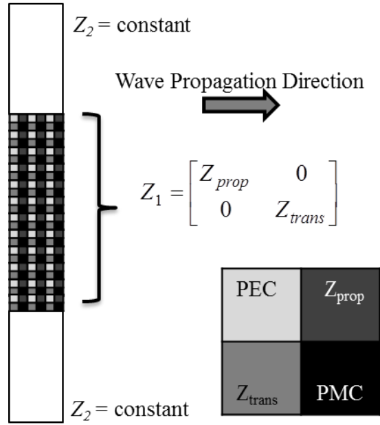
Figure 4.8: Simulation structure of the checkerboard guide. The guide interior is an anisotropic checkerboard surface. The exterior region is an isotropic scalar surface Z_2 = j133\Omega . The guide drawing is not to scale. The details of the checkerboard are replotted (another version is also shown in Figure 4.4). The vacuum height above the surface is 45mm, and the unit cell size is 0.1mm by 0.1mm. The width of each guide was set to 18mm which required 180 unit cells (only 12 unit cells are shown in the figure).
