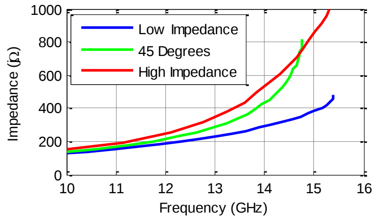
Figure 5.8: Impedance vs. frequency for ring-mushroom unit cell.
