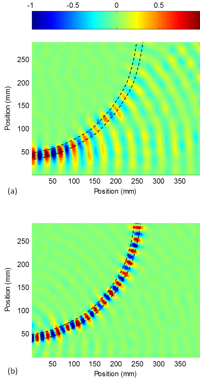
Figure 4.31: Measured fields of curved waveguide. The plots show normalized electric field for guided mode at (a) 11 GHz , and (b) 12 GHz. Fields in (a) and (b) are not plotted to the same scale.
