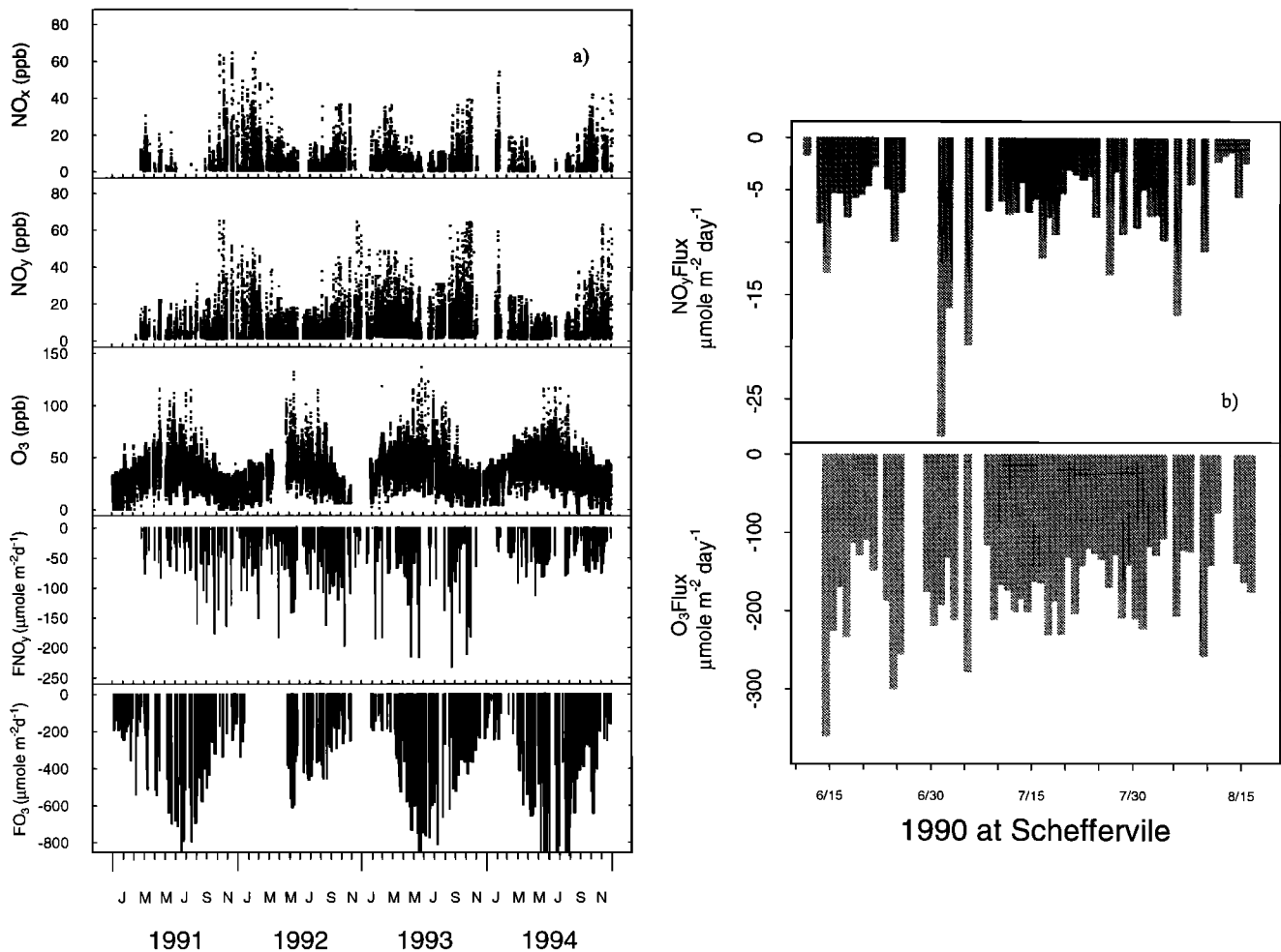
Figure 5. (a) Hourly average concentrations of NO x , NO y , and O 3 and daily integrated fluxes of NO y and O 3 are shown for the period January 1991 to December 1994. The data for 1990, which have more gaps, are not shown. The plot of O 3 concentrations includes results from the profile instrument to fill in periods when the eddy instrument was not working. Instrument problems described in section 2.3 led to frequent gaps early in the sequence. Data recovery improved considerably over the course of the measurements. Fluxes on days with less than 4 missing hours were computed by interpolating between adjacent valid observations. Days with longer gaps were rejected. (b) Integrated daily fluxes of NO y and O 3 are shown for the ABL 3b campaign at Schefferville during summer 1990.
