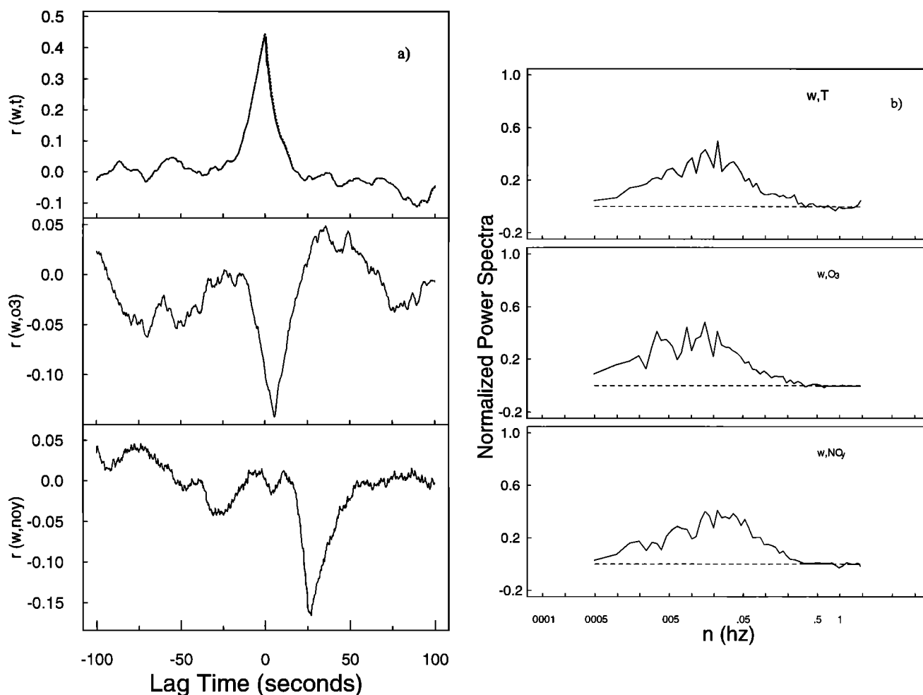
Figure 3. (a) Covariance of vertical wind speed with temperature (top panel), O 3 (middle panel) and NO y (bottom panel) versus time offset. The covariance peak occurs at the lag time corresponding to transit time for air in the sample lines. The data shown are from 1300 (EST), September 13, 1992. (b) Normalized cospectra of T (top panel), O 3 (middle panel), and NO y (bottom panel) with vertical wind are shown versus frequency. The plots are averages of cospectra computed each afternoon for 9 days, September 7-15, 1992.
