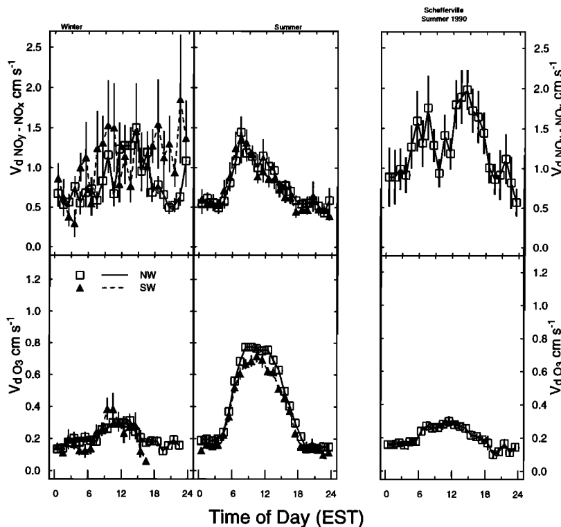
Figure 11. Mean deposition velocities computed for NO y -NO x and O 3 from winter and summer data at Harvard Forest and summer 1990 at Schefferville are shown against hour of the day. Data are conditionally averaged as for Figure 8. In addition, periods with O 3 < NO y are excluded to avoid periods when O 3 chemical reactions may exceed O 3 deposition.
