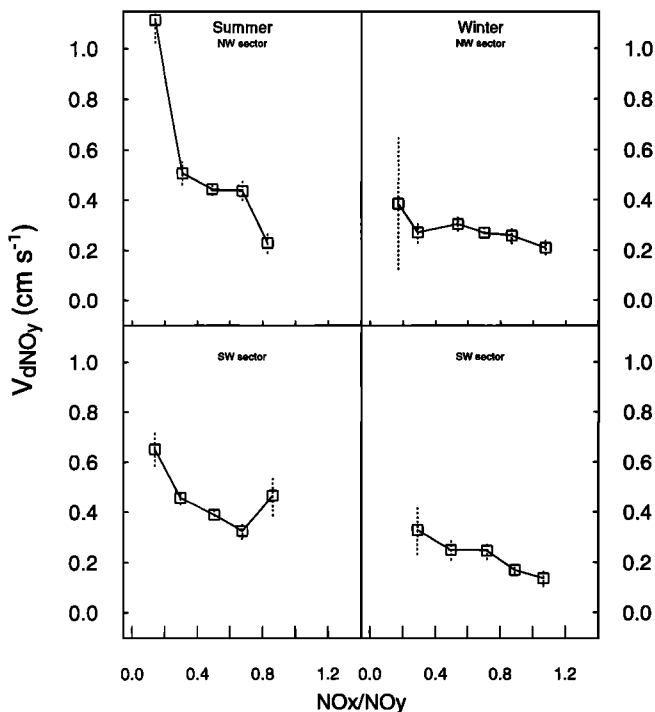
Figure 10. Mean NO y deposition velocity is shown versus NO x /NO y for selected intervals of u* and wind sectors. Vertical segments represent the standard errors about the mean.
