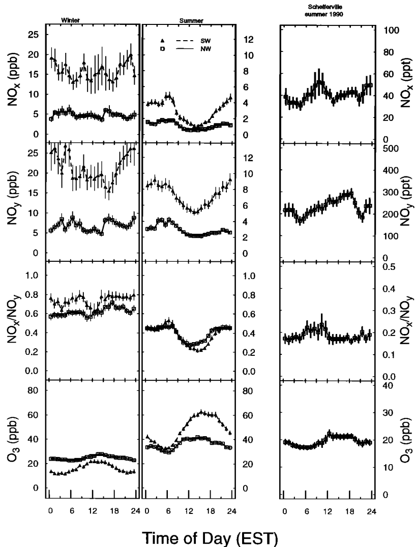
Figure 8. Mean diel cycles of NO x , NO y , NO x /NO y , and O 3 for winter (December - February) at Harvard Forest, column 1, and summer (June - August) at Harvard Forest, column 2, are shown for two dominant wind sectors: 270° - 45° (clean sector) is solid line and open square; 180° - 270° (polluted sector) is long-dashed line and solid triangle. Data for the period March 1990 - December 1994 are used. Vertical bars indicate the standard error about the mean. Very stable or unusually stormy periods are rejected by using only data for 0.1 < u^* < 1.5 and 0.1 < u^* < 1 \text{ m s}^{-1} for winter and summer, respectively. Note the change of scale for NO x and NO y concentrations at Harvard Forest between winter and summer. Mean diel cycles \pm standard error, for Schefferville are shown for the same conditions of u^* ( 0.1 < u^* < 1 \text{ m s}^{-1} ) in column 3. Note the change in scale.
