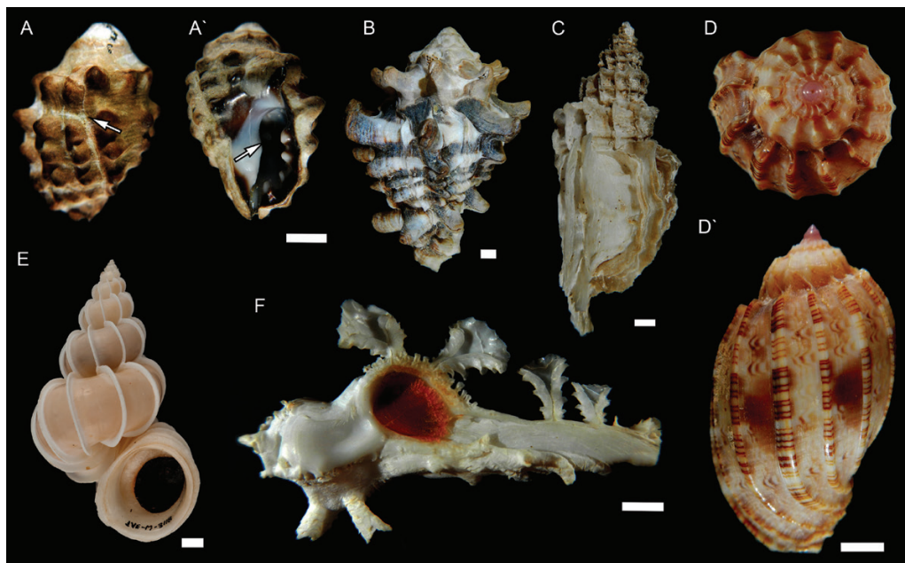
Figure 3. Varix-like sculpture not considered to be a true varix. (A) Ergalataxinae: Tenguella granulata (Duclos, 1832) dorsal view, with scar-like rib (arrow). (A') Apertural view, showing previous apertural teeth associated with scar-like rib (arrow). (B) Vasum turbinellus (L., 1758), dorsal view. (C) Trophoninae: Nipponotrophon stuarti (E. A. Smith, 1880), lateral view. (D) Harpidae: Harpa amouretta Röding, 1798, apical view. (D') Dorsal view. (E) Epitoniidae: Epitonium scalare (L., 1758), JVM3118, apertural view. (F) Muricopsinae: Homalocantha anatomica (Perry, 1811), apertural view. Scale bars: 5 mm. JVM and O represent the University of Alberta collection specimen numbers, specimens without collection numbers come from the Vermeij collection.
