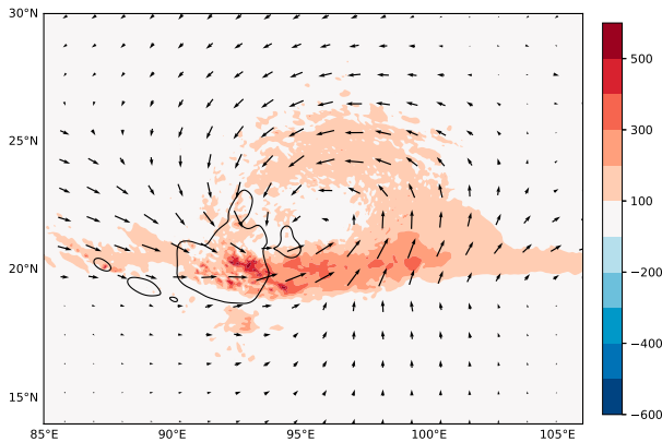
FIG. 7. Perturbation surface latent heat fluxes (shading; \text{W m}^{-2} ), total rain rate (smoothed 5 \text{ mm h}^{-1} contour), and perturbation near-surface winds (vectors) for the same experiment as shown in Fig. 6 at hour 117.
