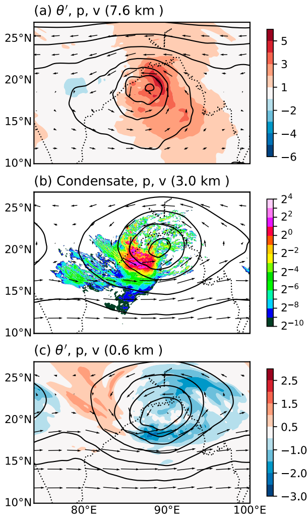
FIG. 4. Sample monsoon depression from \zeta_0 = 1.5 , S_L = -1.0 , and S_U = -2.0 at hour 78. (a) Perturbation potential temperature (shading; \theta' ; K), total pressure (contoured every 0.75 hPa with a minimum contour of 395.25 hPa), and wind vectors at 7.6 km. (b) The vertically integrated condensate from the surface to 15 km (shading; q_c + q_i + q_s + q_r ; \text{g kg}^{-1} ), total pressure (contoured every 2.0 hPa with a minimum contour of 699.0 hPa), and wind vectors at 3.0 km. (c) As in (a), but at 0.6 km with pressure contoured every 2.0 hPa with a minimum contour of 928.0 hPa. The background map is for scale reference only and has no effect on the simulations.
