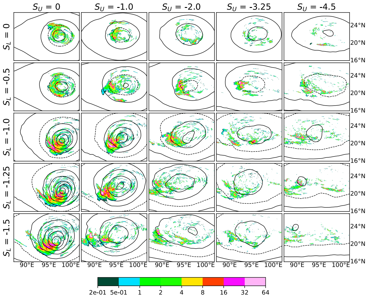
FIG. 10. Rain rate (shading; \text{mm h}^{-1} ) and total pressure (contoured every 1.5 hPa) for all experiments with \zeta_0 = 1.0 for various values of S_L and S_U at day 4.5 of the simulation. The 842 hPa isobar is dashed for ease of comparison.
