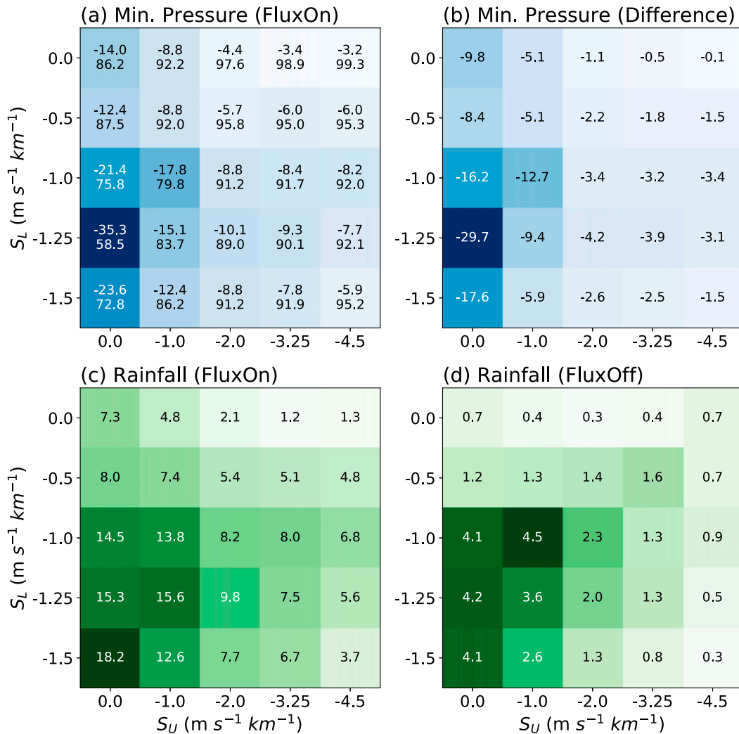
FIG. 8. Summary statistics for experiments with \zeta_0 = 1.0 for various values of S_L and S_U . (a) The minimum pressure reached for the second half of the FluxOn simulation (hPa). Pressure is given as both the perturbation value at 1.5 km (upper number) and the total value at the surface (lower number), expressed without the first digit (e.g., 983.7 hPa = 83.7). (b) The difference between FluxOn and FluxOff for the perturbation pressure shown in (a). (c) The 3-day accumulated rainfall for the second half of the FluxOn experiment (mm). Each value is the average within a 10^\circ \times 10^\circ box centered on the minimum perturbation pressure at 1.5 km. (d) As in (c), but for FluxOff. All values are the average of the two vortices. Note the difference in color scales between (a) and (b) and between (c) and (d).
