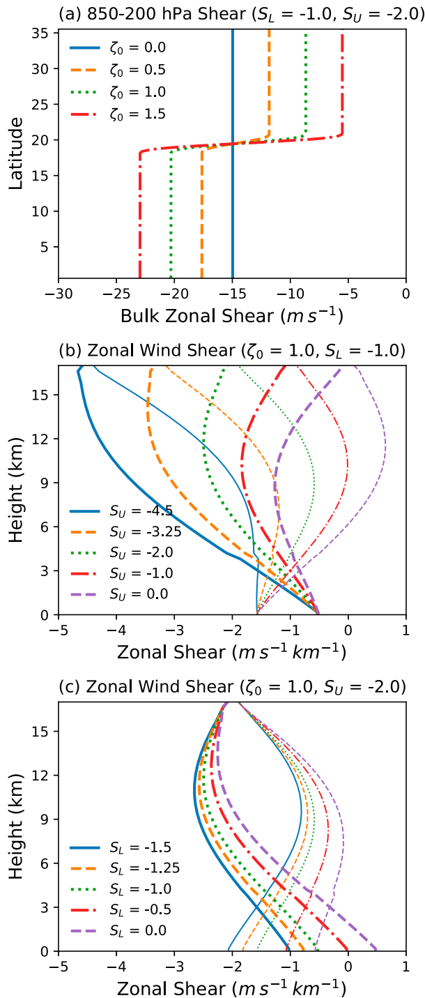
FIG. 2. Basic-state vertical wind shear for various combinations of \zeta_0 , S_L , and S_U . (a) The 850–200 hPa basic-state zonal wind shear ( \Delta\bar{U} ; \text{m s}^{-1} ) as a function of latitude. (b),(c) Basic-state vertical shear of the zonal wind ( \partial_z\bar{U} ; \text{m s}^{-1} \text{km}^{-1} ) as a function of height. The thick lines show profiles south of the monsoon trough axis (which lies at 20^\circ\text{N} ) and the thin lines show profiles north of this axis, both within the regions where vertical shear is constant with latitude, as shown in (a).
