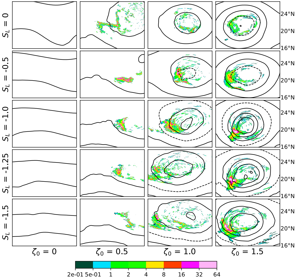
FIG. 12. As in Fig. 10, but for variations in \zeta_0 and S_L .
