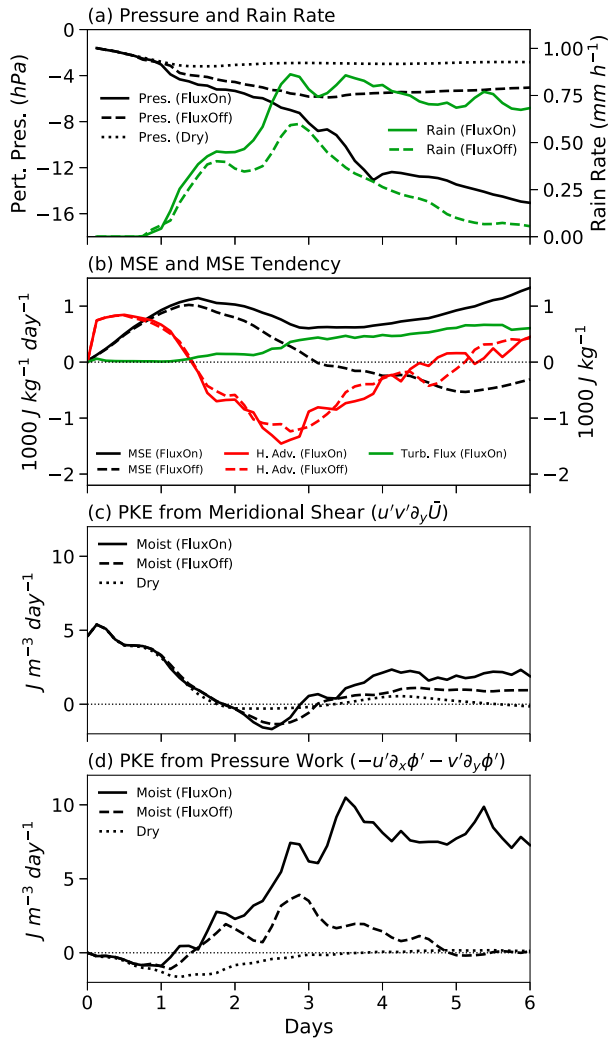
FIG. 5. Time series of various metrics over the life cycle of the vortex for \zeta_0 = 1.0 , S_L = -1.25 , and S_U = -1.0 . (a) Minimum perturbation pressure at 1.5 km (black; hPa) and rain rate (green; \text{mm h}^{-1} ). The solid lines are for FluxOn, the dashed lines for FluxOff, and the dotted lines for Dry. (b) Select terms in the vertically integrated MSE budget. Solid lines are for FluxOn and dashed lines are for FluxOff. The black lines show total perturbation MSE ( 1000 \text{ J kg}^{-1} ), the red line shows total horizontal MSE advection [ 1000 \text{ J kg}^{-1} ; first two terms on right-hand side of Eq. (6)], and the green line shows MSE tendency from surface heat fluxes [last term on right-hand side of Eq. (6)]. (c) The meridional shear term ( u'v'd_y\bar{U} ) in the PKE equation. The solid line shows FluxOn, the dashed line shows FluxOff, and the dotted line shows Dry. (d) As in (c), but for the pressure work term.
