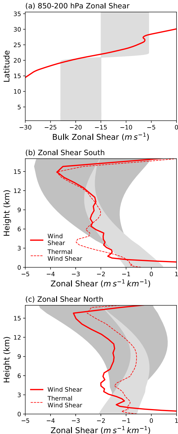
FIG. 3. Profiles of vertical shear of the zonal wind for a pregenesis composite of monsoon depression environments compared with those shown in Fig. 2. (a) As in Fig. 2a, but for the composite profile (red line). The gray shading indicates the ranges of values shown in Fig. 2a, but shifted to be centered at 21°N. (b),(c) Basic-state vertical shear of the zonal wind ( \partial_z \bar{U} ) as a function of height for the composite profile (red line). The gray shading indicates the ranges
