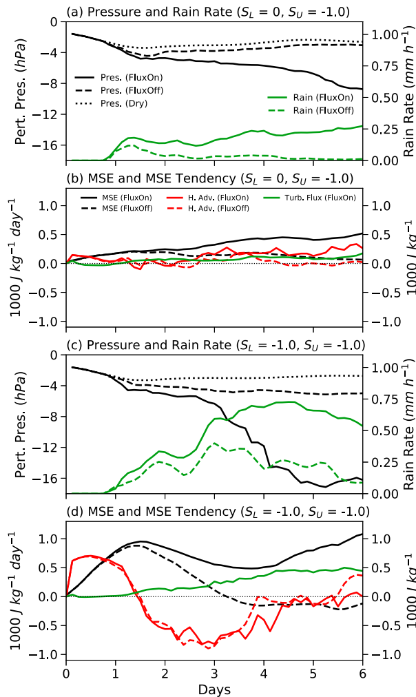
FIG. 9. Time series comparison of pressure, rain, and MSE for two experiments. (a),(b) As in Figs. 5a and 5b, but for \zeta_0 = 1.0, S_L = 0.0 , and S_U = -1.0 . (c),(d) As in (a) and (b), but for S_L = -1.0 .
