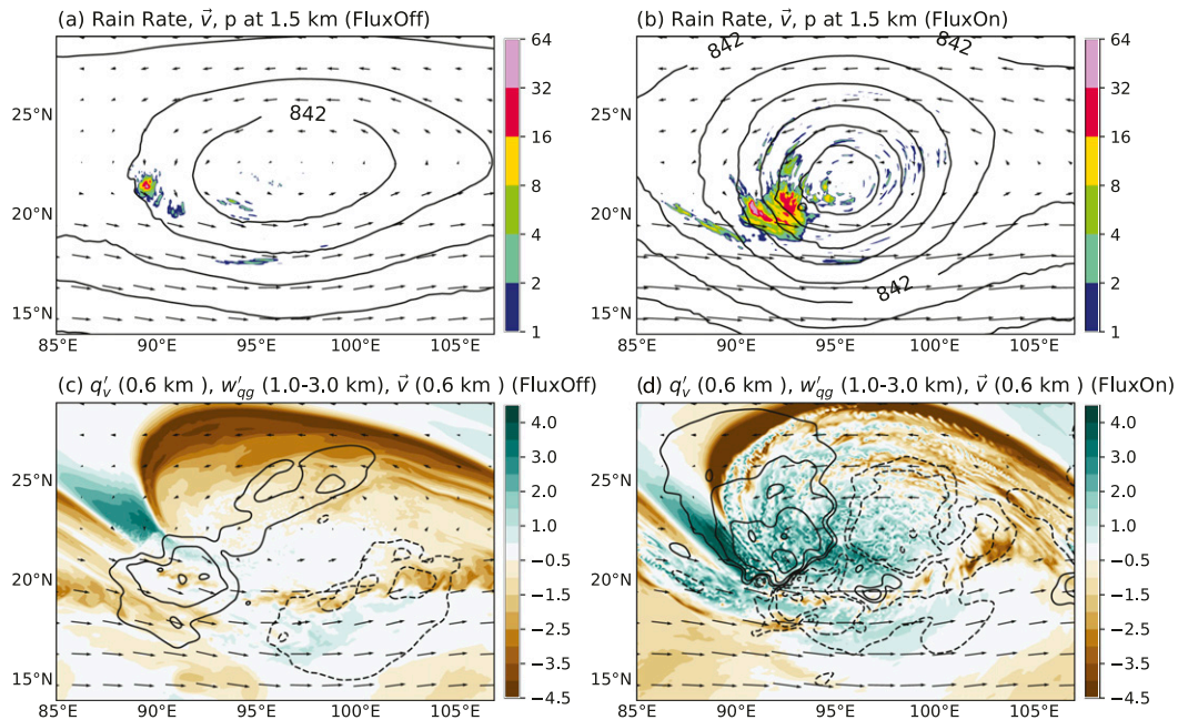
FIG. 6. Comparison between (a),(c) FluxOff and (b),(d) FluxOn for \zeta_0 = 1.0 , S_L = -1.25 , and S_U = -1.0 at hour 117. (a),(b) Hourly rain rates over the previous three hours (shading; \text{mm h}^{-1} ), total pressure at 1.5 km (contoured every 1.5 hPa with the 842 hPa contour labeled), and total wind (vectors; \mathbf{v} ; 1.5 km). (c),(d) Perturbation mixing ratio (shading; q'_v ; \text{g kg}^{-1} ; 0.6 km), perturbation vertical velocity from the QG omega equation (contoured on a log-2 scale beginning at 0.5 \text{ cm s}^{-1} and smoothed with a Gaussian filter, with upward motion in solid contours), and total wind (vectors; \mathbf{v} ; 0.6 km).
