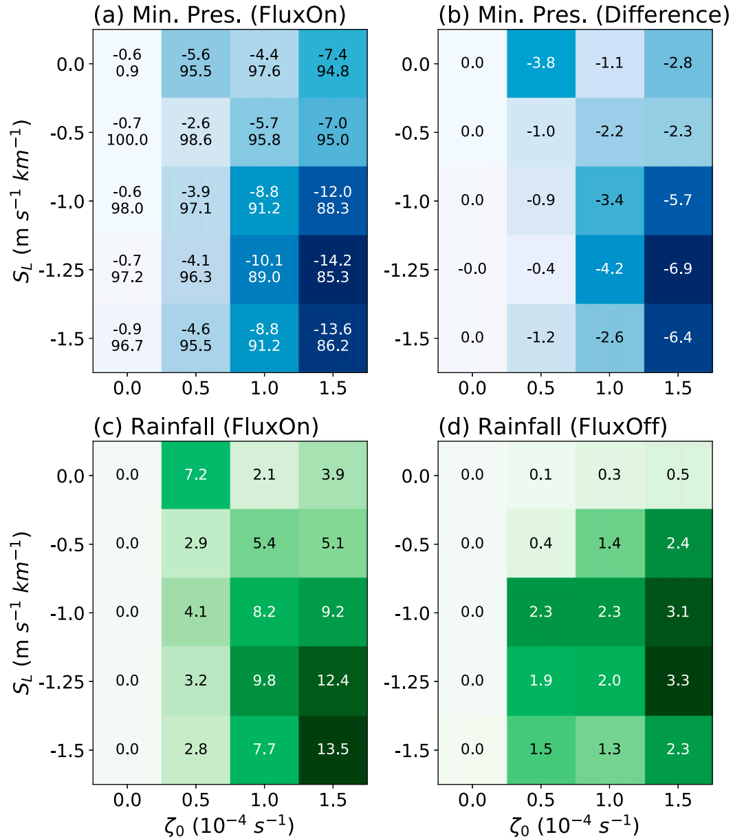
FIG. 11. As in Fig. 8, but for variations in \zeta_0 and S_L .
