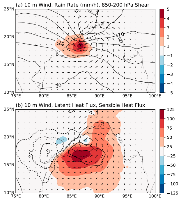
FIG. 1. Composite monsoon depression from ERA5 based on the 1982–2018 IMD track dataset. (a) Anomalous surface precipitation rate (shading; \text{mm h}^{-1} ), 850–200 hPa vertical shear of the zonal wind (contours; \text{m s}^{-1} ), and anomalous 10 m wind (vectors). (b) Anomalous surface latent heat flux (shading; \text{W m}^{-2} ), anomalous surface sensible heat flux (contoured every 10 \text{ W m}^{-2} , excluding zero), and anomalous 10 m wind (vectors). All anomalies are from the time-mean climatology.
