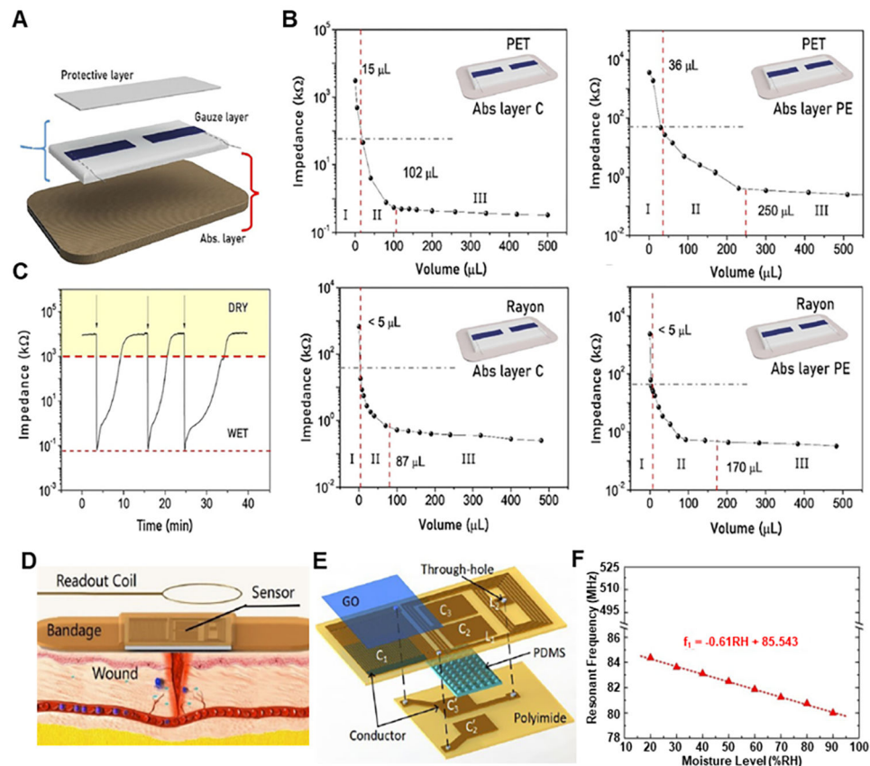
Figure 8. Wearable moisture sensing devices for wound healing. (A) Schematic of bandage sensor showing three different composition layers. (B) Bandage sensor response to the addition of synthetic exudate. (C) Real-time monitoring of the sensor's impedance when the status switches between wet and dry, showing a reversible behavior. Reproduced under the terms and conditions of the CC BY [72] . Copyright 2021, The Author(s), published by Frontiers. (D) Conceptual diagram of wireless moisture sensor integrated with bandage for wound monitoring. (E) Structural diagram of designed LC-type wireless pressure and moisture sensor. (F) Measured resonant frequencies when RH changes from 20% to 90%. Reproduced with permission [73] . Copyright 2018, IEEE.
