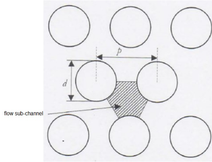
Figure 4.8: Triangular Lattice
