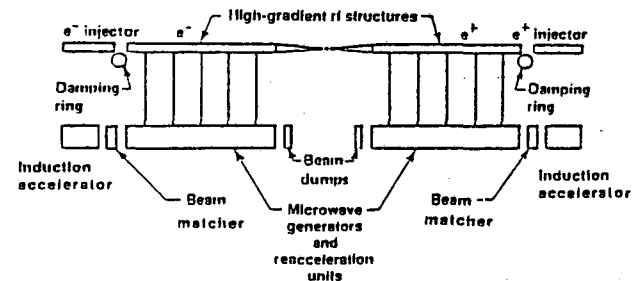
Fig. 1. Schematic of a Two-Beam Accelerator. The low energy drive beam provides power to the high energy beam. Reacceleration is provided by induction units or with superconducting RF cavities. Conversion of beam energy to microwaves is provided by either relativistic klystrons or free-electron lasers.
