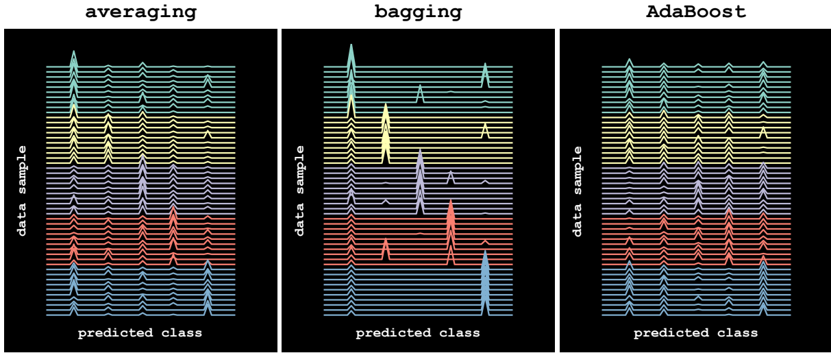
Figure 4.5. Diversity plots for JSC.S. While AdaBoost is very diverse, the high peak density off the diagonal shows that many ensemble members classify incorrectly. Averaging best balances diversity with correctness.
