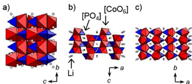
Fig. 1 Projections of the crystal structures of olivine-type \text{LiCoPO}_4 (space group Pnma ) along the three crystallographic axes: (a) [100], (b) [010], and (c) [001]. [\text{CoO}_6] octahedra are drawn in red, [\text{PO}_4] tetrahedra in blue, and Li ions in grey.
