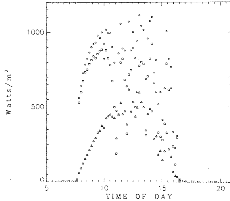
Fig. 5. The time dependence of various parameters of the solar radiation on December 23, 1976 in Albuquerque, New Mexico showing the normal incidence readings from the pyr heliometer (□), and the total radiation readings from the horizontal pyranometer (△) and from the sun tracking pyranometer (○).
