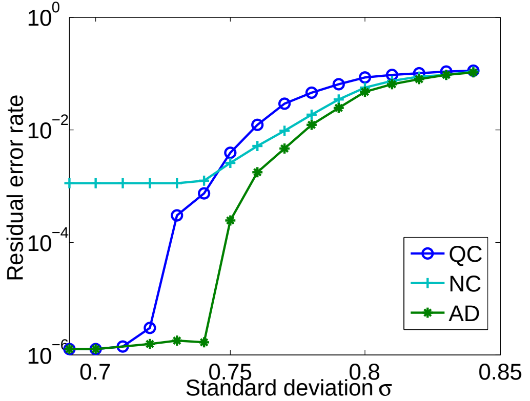
Figure 4.10: Comparison of residual error rates under NC, QC, and AD for different \sigma in finite length code simulations.
