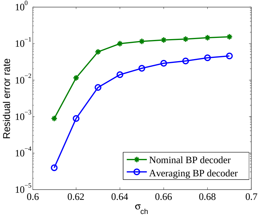
Figure 3.6: Residual error rate comparison with \sigma_{cmp} = 3 .
