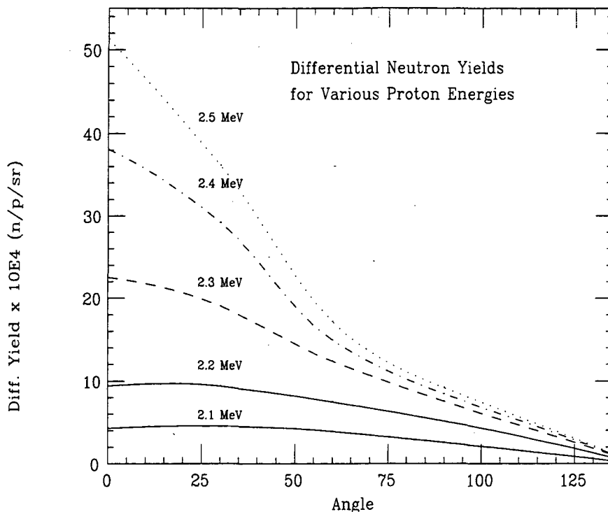
Figure 2.1: Differential neutron yields for protons on a thick {}^7\text{Li} metal target.
