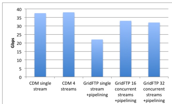
Figure 13: GridFTP vs. Climate Data Mover (CDM)
