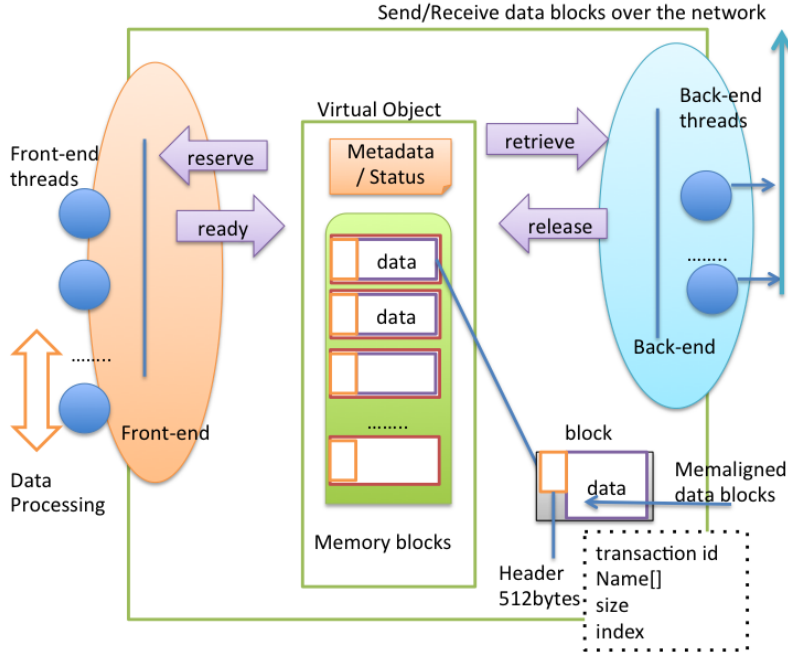
Figure 9: Climate Data Mover Framework
