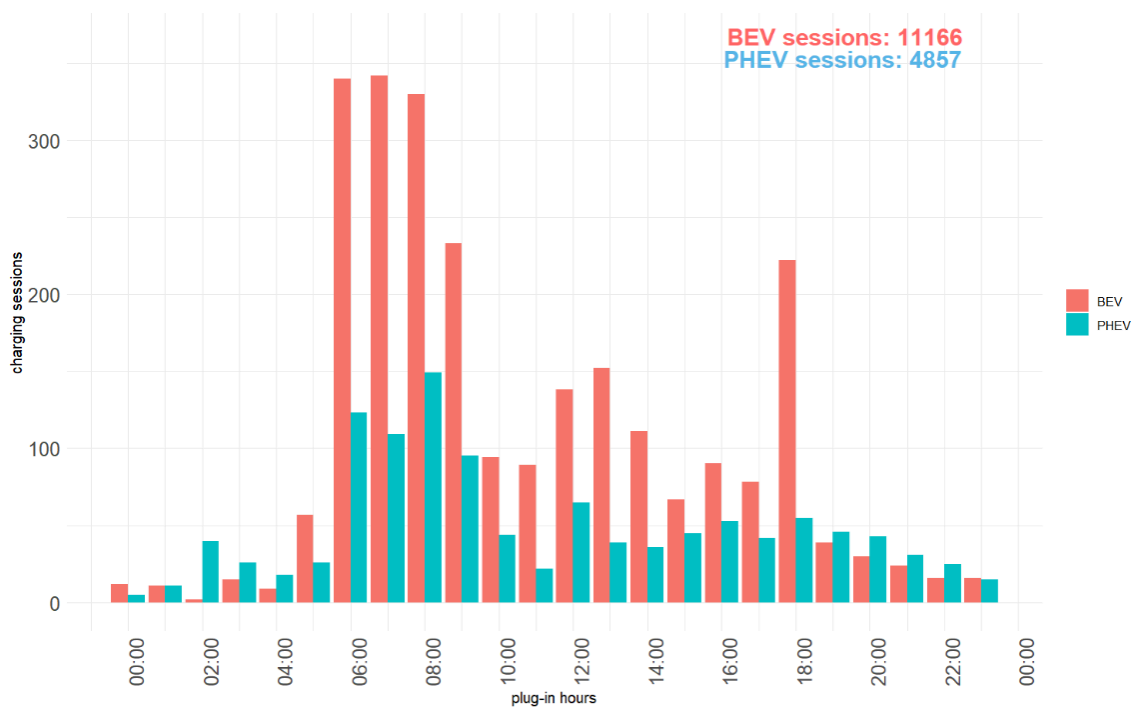
Fig 12. Average vehicle charging sessions by plug-in time and vehicle type.
