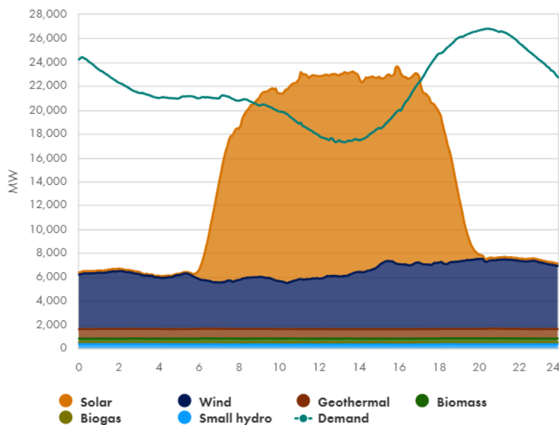
Fig 4. California's renewable energy supply and demand (in megawatts) over 24 hours, with every 5-minute daily increment data, on June 1, 2024.
