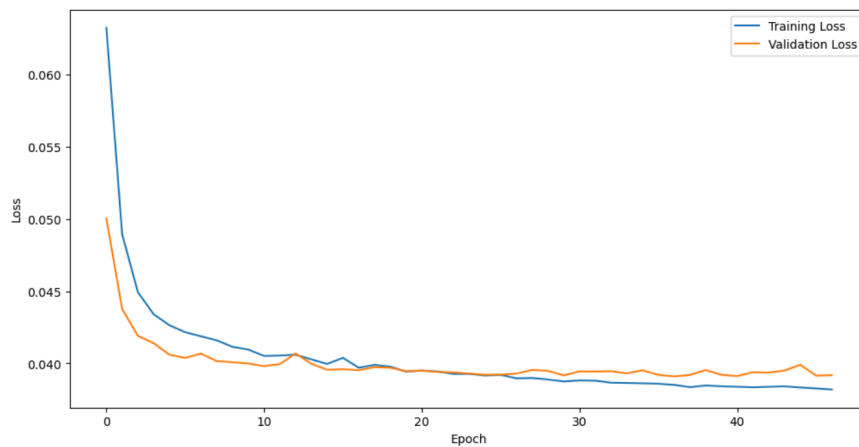
Fig 25. Training and validation loss curve with 40 epoch
