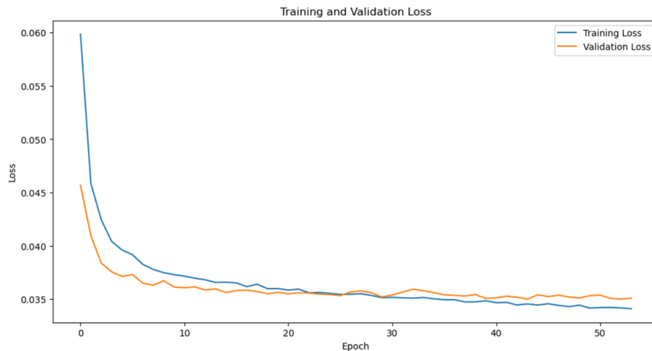
Fig 26. Training and validation loss curve with 50 epoch
