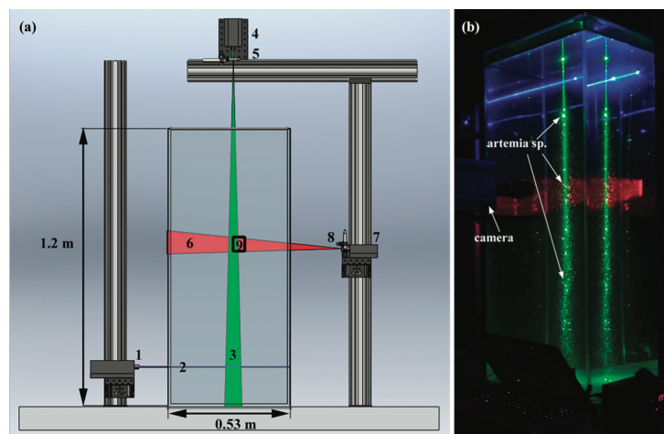
Figure 1: Experimental setup by Wilhelmus and Dabiri (2014). Laser guidance system for control of animal migrations. A 447 nm laser (1) generates a horizontal blue laser beam (2) aligned with a vertical green laser sheet (3), generated by a 532 nm laser (4), and introduced from above the tank through a 25 mm focal length cylindrical lens (5), and a vertical, red laser sheet (6) is utilized for PIV measurements.
