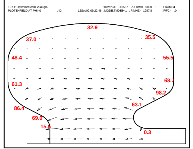
Figure 1: Cavity Wall Power Density, Watts/cm 2 , see text
