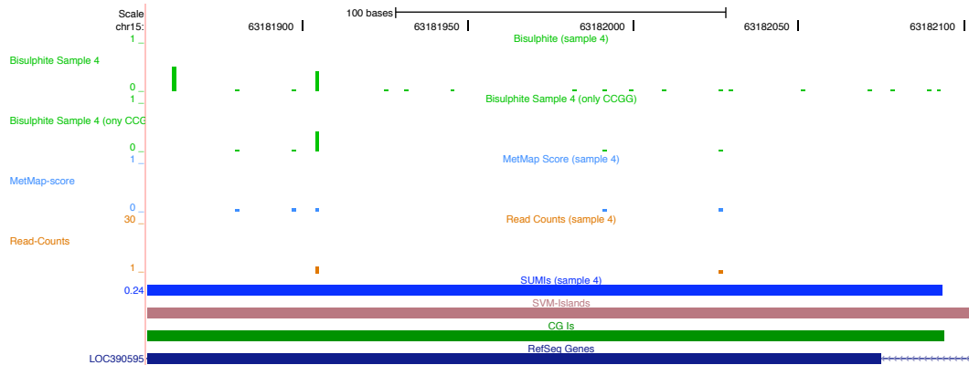
(s) chr15-63,181,854-63,182,103
