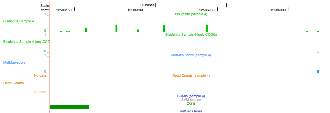
(u) chrY-12,586,134-12,586,330
