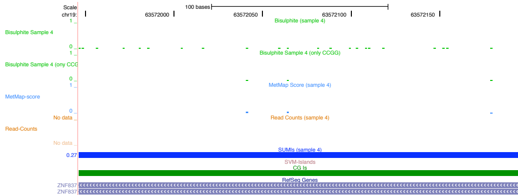
(t) chr19-63,571,947-63,572,196
