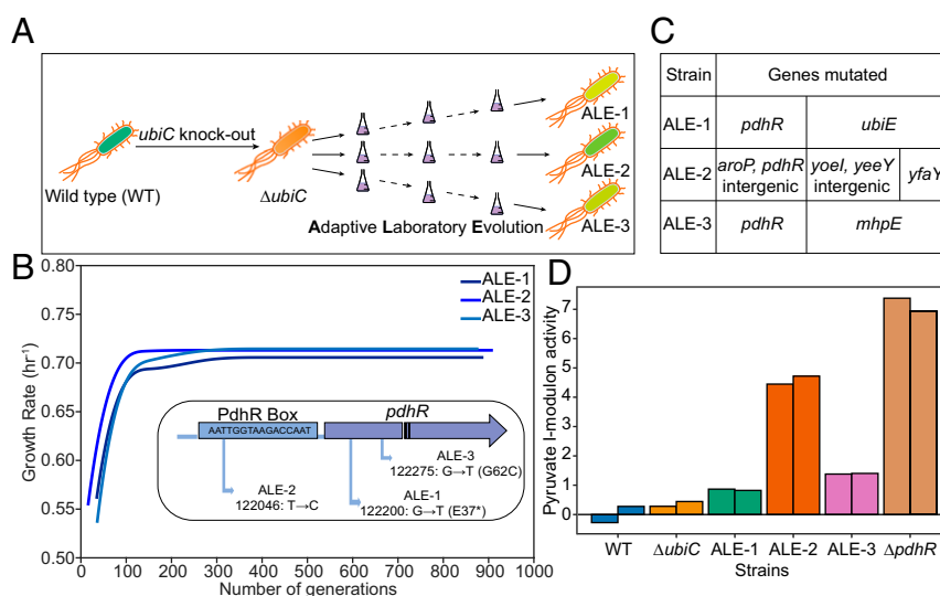
Fig. 1. Experimental evolution of E. coli \Delta ubiC strain. (A) The schematic for generation of strains used in the study. (B) The growth rate evolution trajectories (smoothed data) and the convergent mutations ( Inset ) observed in \Delta ubiC replicates during laboratory evolution. SI Appendix, Fig. S1C shows the extended axis plot of these trajectories. (C) List of genes mutated during the evolution of the \Delta ubiC replicates. (D) Activity of the pyruvate i-modulon estimated by independent component analysis (ICA). \Delta pdhR has been used as the control strain. The bars with identical colors represent biological replicates of the corresponding strain.
