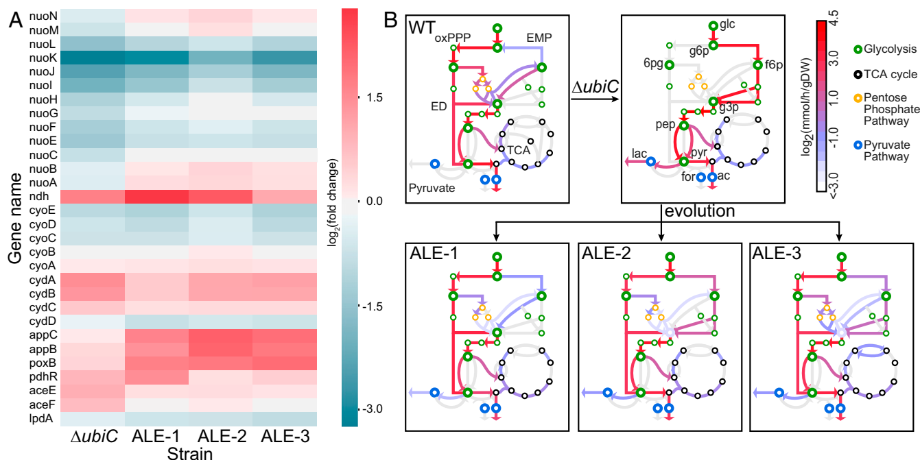
Fig. 2. Evolutionary optimization of the respiratory system. (A) Heatmap showing the expression changes of enzymes involved in ETS and pyruvate metabolism. Fold-changes have been calculated with respect to the wild-type strain. (B) Computed metabolic flux maps depict the differences in central metabolism between the WT, the preevolved, and evolved strains (ALE-1, 2, and 3). Major pathways represented in the figure include glycolysis (metabolites colored in green), oxidative pentose phosphate pathway (oxPPP, yellow), the TCA cycle (black), and the pyruvate pathway (blue). Key metabolites are indicated in the figure as follows: glc, glucose; g6p, D-glucose-6-phosphate; g3p, glyceraldehyde-3-phosphate; f6p, D-fructose-6-phosphate; pyr, pyruvate; 6pg, 6-phospho-D-gluconate; pep, phosphoenolpyruvate; lac, lactate; for, formate. Calculated fluxes of each strain are colored on a log scale.
