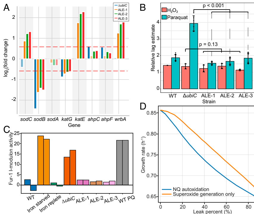
Fig. 3. Oxidative stress mitigation. (A) Expression changes in ROS-quenching enzymes. Fold-changes have been calculated with respect to the wild-type strain [periplasmic superoxide dismutase, sodC ; cytosolic superoxide dismutase, sodB and sodA ; bifunctional hydroperoxidase, katG ; monofunctional catalase, katE ; alkyl hydroperoxide reductase, ahpC and ahpF ; NAD(P)H:quinone oxidoreductase, wrbA ]. (B) Estimation of the growth retardation caused due to addition of peroxide (1 mM H 2 O 2 ) and superoxide (1 μM paraquat) generating chemicals by calculating the relative increase in the lag phase. For each strain, the mean of the estimated lag phase across untreated replicates (control) was calculated. The lag-phase estimates of the conditions with treatment was then divided by the corresponding control condition (yielding the relative lag phase). The error bars represent the SD for the lag estimates across replicates ( n \geq 3 ). The effect of adaptive evolution was significant in the paraquat treatment ( P value < 0.001) but not in peroxide treatment ( P value = 0.13) (Materials and Methods). (C) Adaptive changes in the activity of Fur i-modulon in the evolved strains. Iron-starved, iron-replete, and paraquat-treated WT conditions serve as controls. The bars with identical colors represent biological replicates of the corresponding strain. (D) Genome-scale model-based calculation of the impact of periplasmic nonproductive electron leak on the growth rate of E. coli . SI Appendix, Fig. S5 shows the extended axis plot of these calculations.
