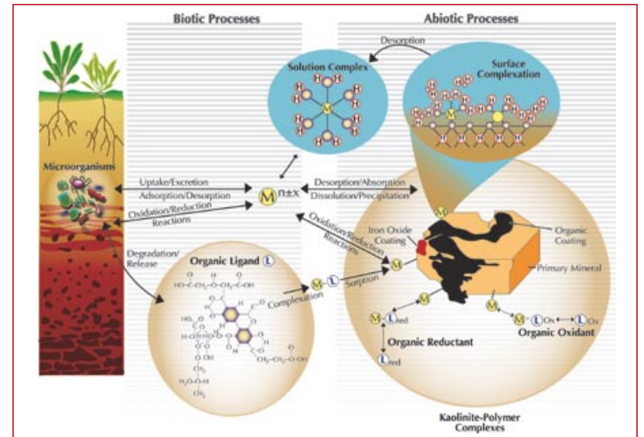
Figure 5.1. Abiotic and biotic mechanisms influence the fate of metals (M) in subsurface environments. From left to right: Organic material produced by microorganisms can act as ligands (L) and complex with metals, facilitating transport. These ligands can also be degraded by microbes to release the metal. Microbes can also directly adsorb/desorb, take up/excrete, and oxidize/reduce metals. Oxidation and reduction will change the valence state of the metal either up or down ( M^{n\pm x} ). Abiotically, metals can form solution complexes or can complex with the surface of clays (kaolinite-polymer complexes). These mineral complexes can sorb metals either directly to the mineral or to organic or iron oxide coatings. Metals can also be directly oxidized or reduced to different valence states by the ambient redox conditions or by organic reductants ( L_{red} ) or oxidants ( L_{ox} ). Changing the valence state of metals will affect their sorption, mobility, precipitation, and toxicity. (Image courtesy of S. Fendorf, Stanford Univ.)
