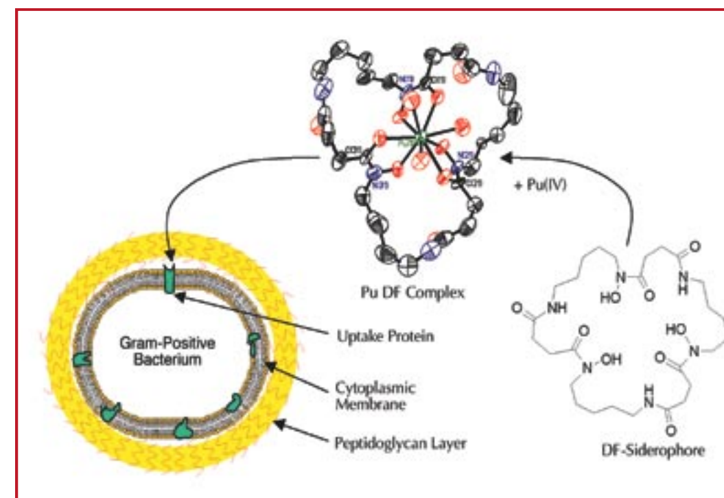
Figure 5.9. Siderophore-mediated Pu accumulation by Microbacterium flavescens (John et al., 2001).
