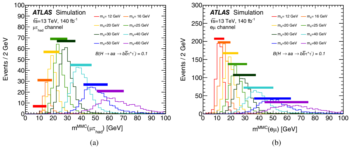
FIG. 6. Mass distribution of the \tau\tau system for each of the generated MC signal mass points for the (a) \mu\tau_{\text{h}} and (b) e\mu categories. The rectangle above each histogram shows the domain used to test each mass hypothesis. Note that nearby mass hypotheses have overlapping regions. All distributions are normalized assuming B(H \rightarrow aa \rightarrow b\bar{b}\tau^+\tau^-) = 10\% .
