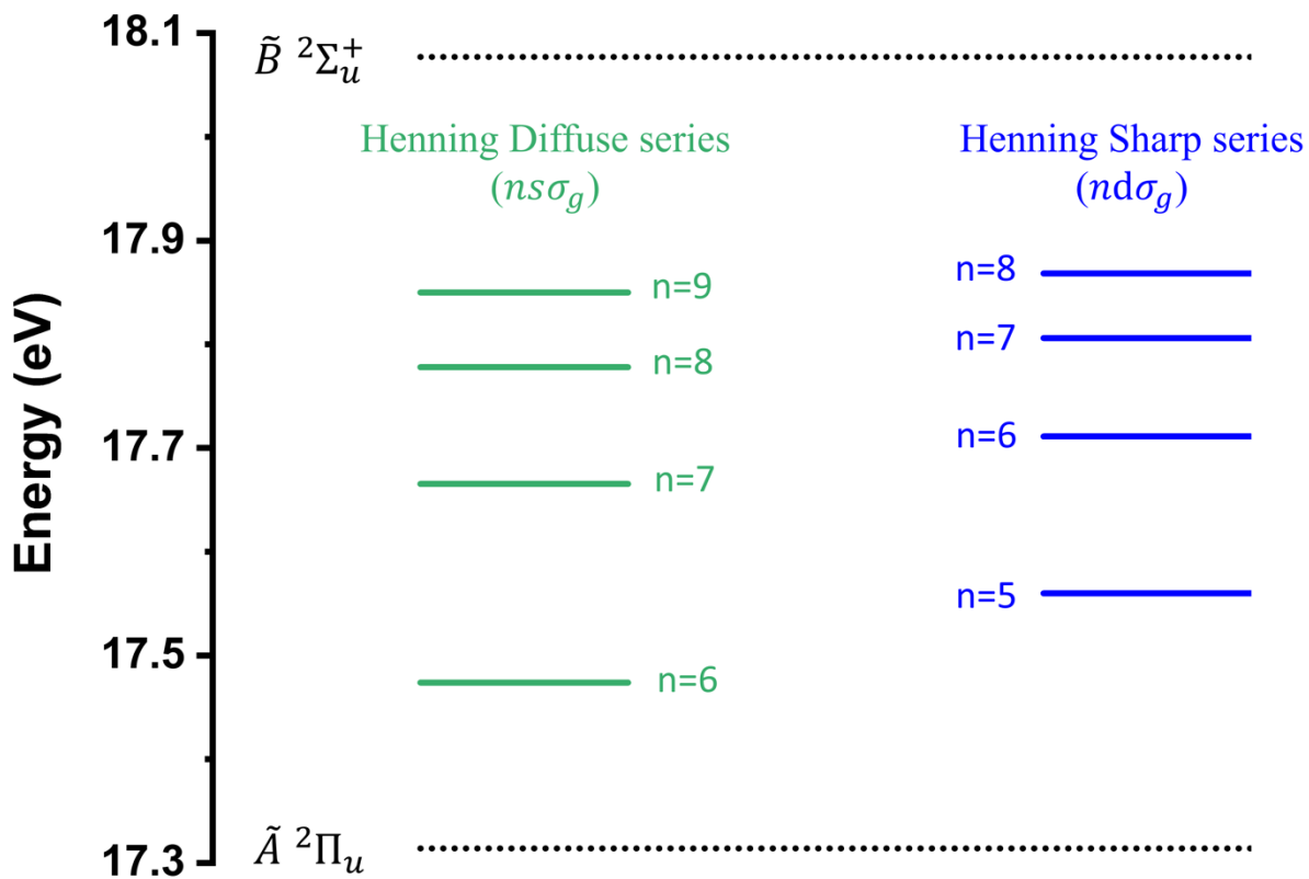
FIG 1: Energy level diagram of the Henning diffuse (green) and Henning sharp (blue) Rydberg series of CO 2 between 17.3-18.1 eV. Dotted lines represent ionic states while solid lines represent neutral Rydberg states. Both the ns\sigma_g character Henning diffuse and nd\sigma_g character Henning sharp series converge to the ionic \tilde{B} \ ^2\Sigma_u^+ state.
