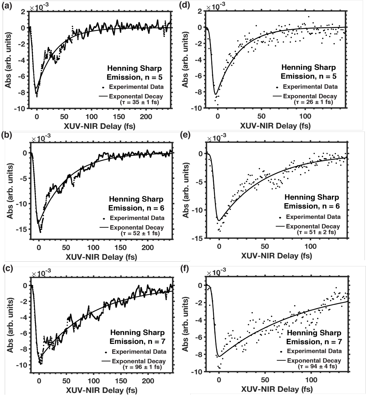
FIG 8: Delay-dependent traces of wave-mixing emission features observed at the energy positions of the Henning sharp (a) n = 5 (17.49 – 17.55 eV), (b) n = 6 (17.66 – 17.70 eV), and (c) n = 7 (17.77 – 17.80 eV) states in dataset #1 and the (d) n = 5 (17.48 – 17.54 eV), (e) n = 6 (17.65 – 17.71 eV), and (f) n = 7 (17.76 – 17.81 eV) states in dataset #2. The dots in each of the panels represent measured experimental data while the solid lines are numerical fits. The time constants and errors provided here correspond to the least squares fit of a single data set. The data points of dataset #1 were interpolated to obtain a constant step size for analysis. The decay constants measured correspond with the lifetimes of the Henning diffuse states, not the sharp states from which they emit.
