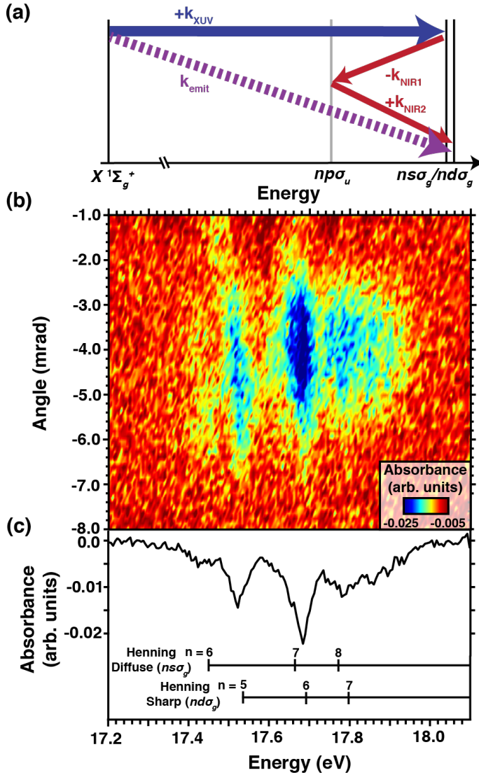
FIG 3: Background-free wave-mixing signals are detected by an X-ray CCD camera at spatial and temporal overlap of all three pulses. (a) A wavevector phase-matching diagram demonstrating the generation of spatially isolated four wave mixing signals (dashed, purple arrow) from an XUV pulse train (thick, blue arrow) and two NIR pulses (thin, red arrows). Not to scale. (b) An X-ray charge coupled device (CCD) image plotted as a function of photon energy and phase-matching divergence angle reveals multiple wave-mixing emission features (blue). (c). An angle-integrated trace taken from this camera image can be compared to literature photoabsorption spectra for spectral assignment. The observed emission features correspond primarily to Rydberg series that converge to the ionic \tilde{B}^2\Sigma_u^+ limit, with the Henning sharp series representing the dominant contribution.
