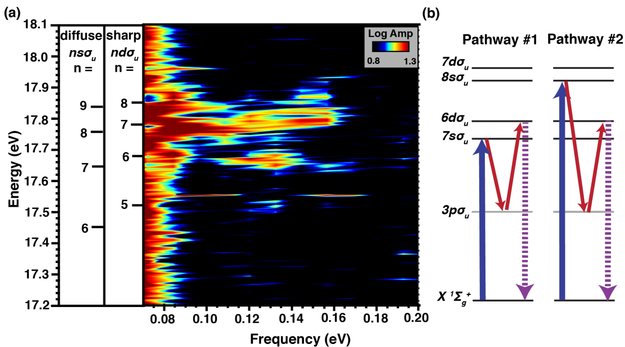
FIG 6: (a) Fourier analysis of the delay-dependent wave-mixing emission spectrum. State assignments are provided to the left of the spectrum. Broad frequency-domain features are observed at energies associated with the Henning sharp series. (b) Interference between wave-mixing pathways built on different Rydberg series members within the XUV bandwidth leads to oscillations with frequencies consistent with those measured in the Fourier transform in the wave-mixing emission spectrum. The NIR pulses are represented by thin, red arrows, while the XUV pulse and FWM emission are represented by thick blue and dashed purple arrows, respectively.
