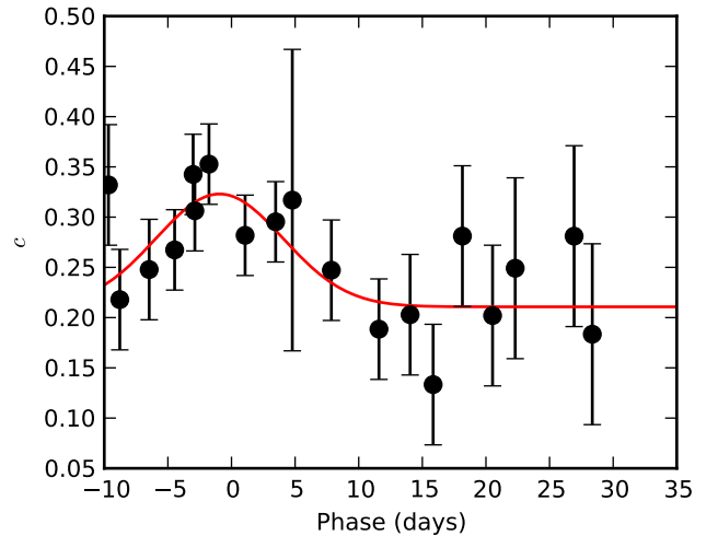
Figure C2. The fitted values of parameter c in after the SED of SN 2011fe has been fitted together with Equation (C1) to match SN 2011by uvm2 photometry. The solid line is showing a Gaussian fit.
