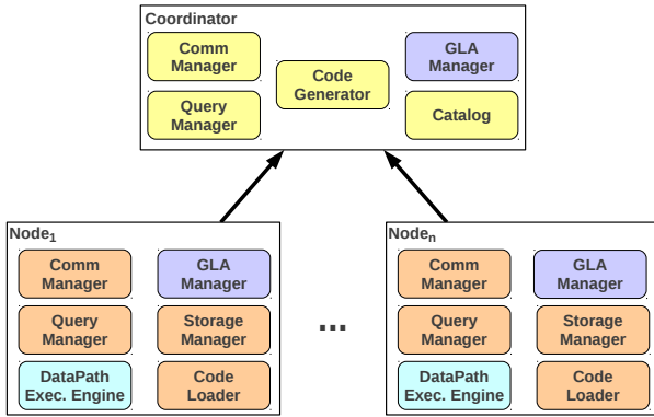
Figure 4: GLADE architecture.
