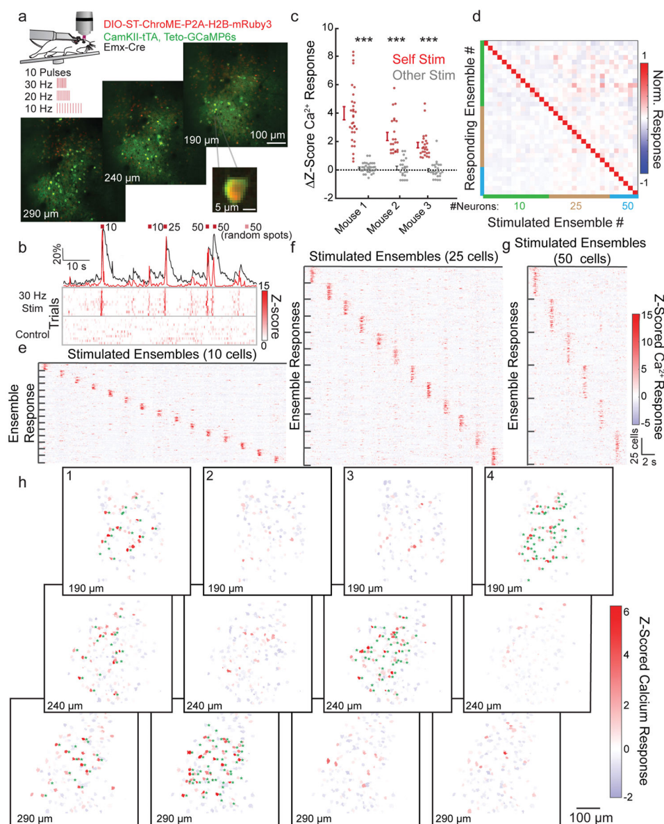
Figure 7. Manipulating neural ensembles with high temporal and spatial precision
