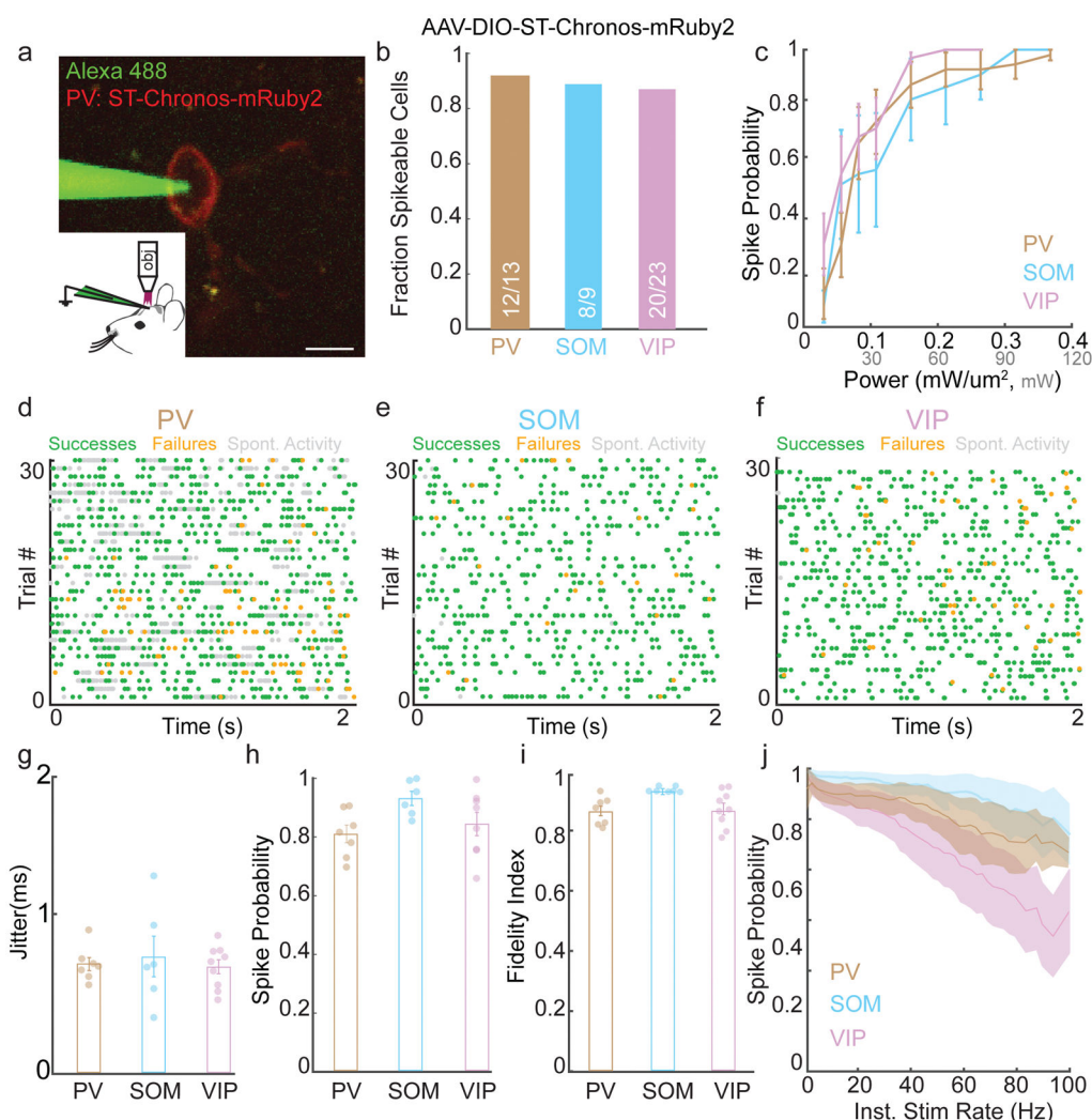
Figure 4. Spatiotemporal activation of cortical inhibition
