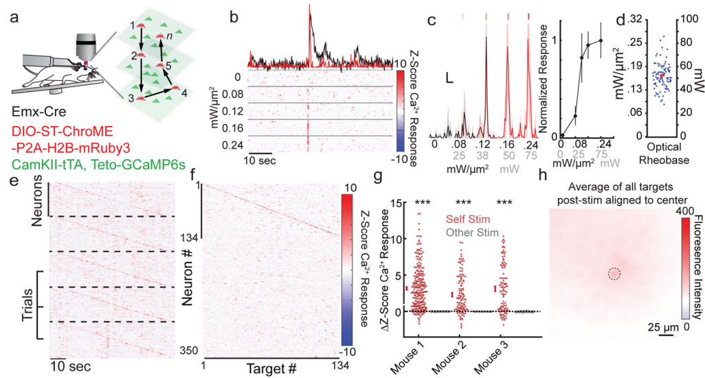
Figure 5. All-optical read/write with high spatiotemporal fidelity
