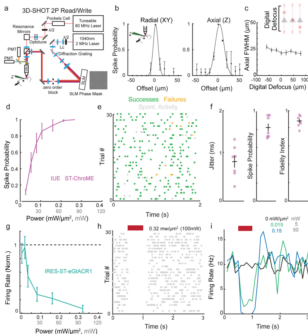
Figure 3. Creating and editing spatiotemporal neural activity in vivo
