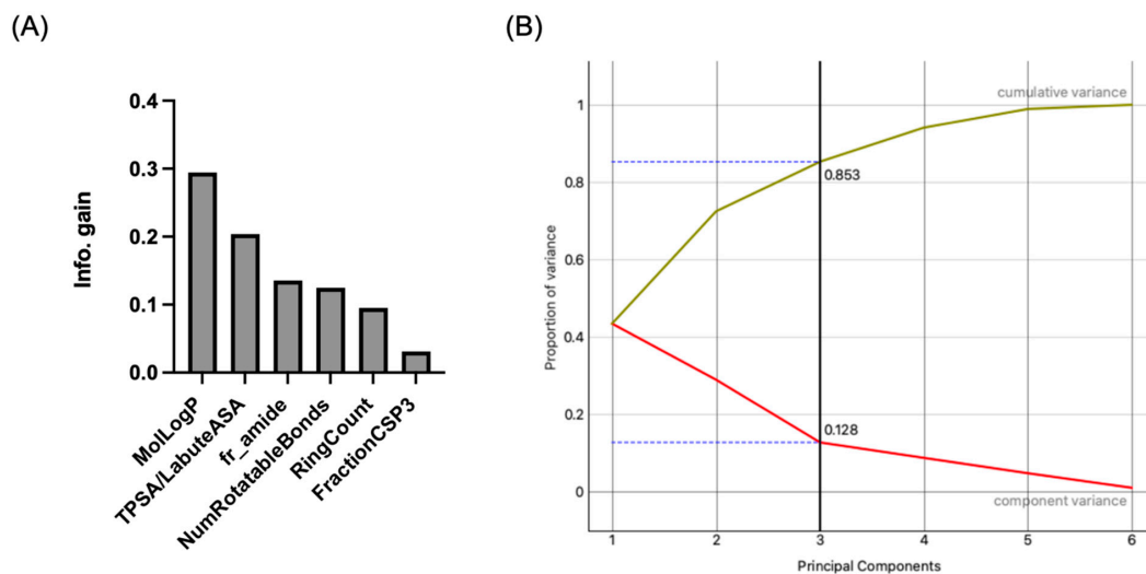
Figure 2. Ranking of molecular properties for binary classification of OAT-interacting and MRP-interacting drugs based on the information gain metric and principal component analysis (PCA). (A) Shown is a bar graph of the molecular properties ranked based on information gain. As described in the text, this was one of several methods used to come up with the final set of molecular properties for binary classification. (B) Principal component analysis indicates that the initial three principal components explain ~85 percent of the variance.
