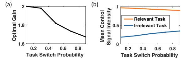
Figure 3: Gain optimization for experiments with different task switch probabilities. (a) The optimal gain is plotted as a function of task switch probability in the experiment sequence. (b) The average intensity of the control unit dedicated to the currently relevant task (orange), as well as the intensity of the control unit associated with the irrelevant task (blue) are shown as a function of task switch probability in a given experiment sequence.
