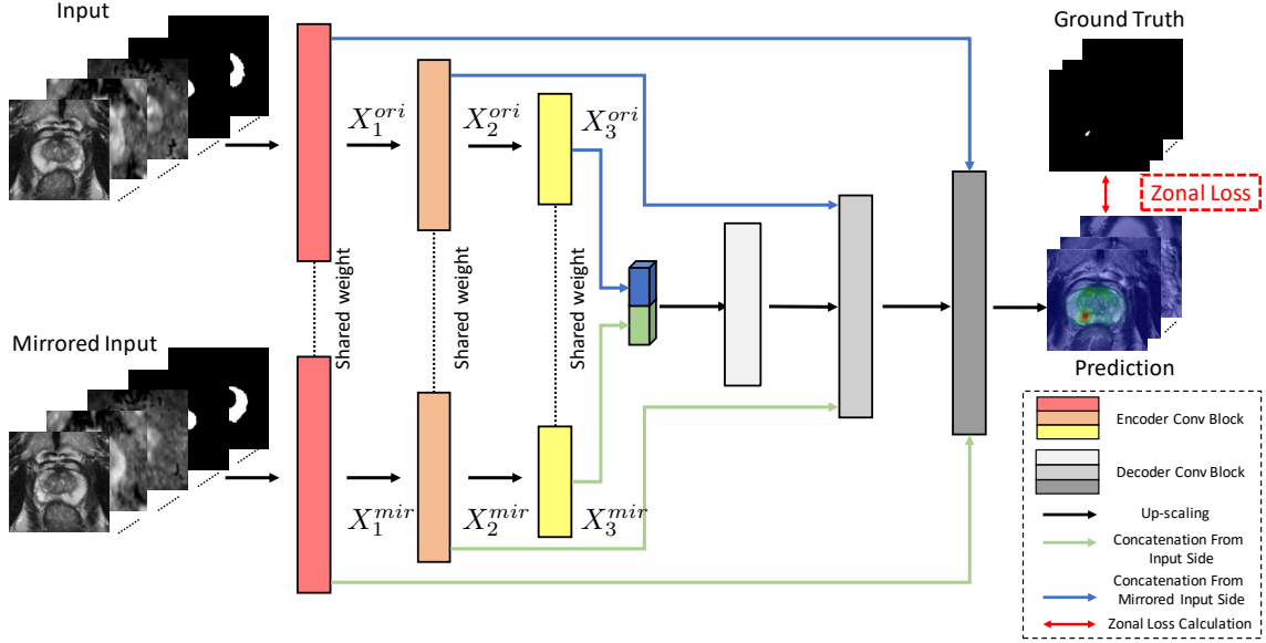
Figure 5.2: Architecture of the proposed AtPCa-Net. It combines the 3D symmetric-aware network and the proposed Zonal Loss (ZL). The network takes input stack images of T2WI, ADC, high-B DWI, TZ’s mask, and PZ’s mask images in an original way and a mirrored way. The weights of encoders at each level from the two sides of the figure are shared. At each level, the feature maps from two sides are concatenated first together and go through a bridge convolution block that consists of two consecutive 3D convolution blocks, then concatenated with the upscaled feature maps from the lower level, and finally upscaled to the upper-level decoder layers.
