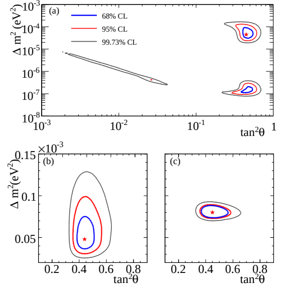
FIG. 2: Neutrino-oscillation contours. (a) SNO only: D 2 O & salt day and night spectra, NCD phase fluxes. The best-fit point is \Delta m^2 = 4.57 \times 10^{-5} \text{ eV}^2 , \tan^2\theta = 0.447 , f_B = 0.900 , with \chi^2/\text{d.o.f.} = 73.77/72 . (b) Solar Global: SNO, SK, Cl, Ga, Borexino. (c) Solar Global + KamLAND. The best-fit point is \Delta m^2 = 7.94 \times 10^{-5} \text{ eV}^2 , \tan^2\theta = 0.447 , f_B = 0.873 .
