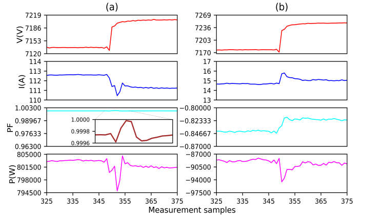
Fig. 5. Response of the two feeders to grid-induced event: (a) response of the solar distribution feeder; (b) response of the auxiliary neighboring feeder.
