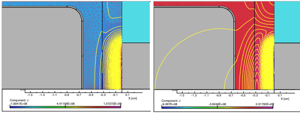
Figure 5: Flux and Eddy Current \omega t = \pi (l), \omega t = 2\pi (r)
