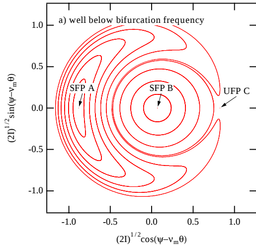
Figure 10: Poincaré map of the phase space in a frame rotating with the modulation frequency when exciting below the below bifurcation frequency.
