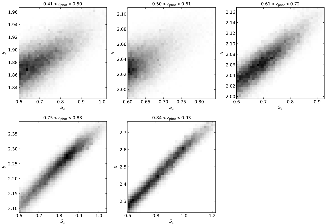
Figure 15. Two dimensional posterior distribution of galaxy bias vs. the photo- z error rescaling factor S_z (a nuisance parameter in our analysis) at different redshifts. The correlations are much stronger at higher redshifts due to the overall larger photo- z errors that dilute the clustering signal.
