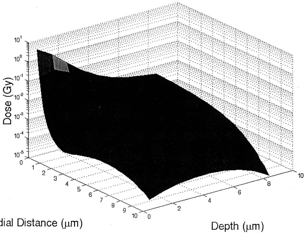
Figures 4.1 – 4.3: 3-D plots of dose distributions D(r,x) in (Gy) as function of radial distance ( r ) and of penetration ( x ) for each code: PENELOPE, MCNP, PITS.
