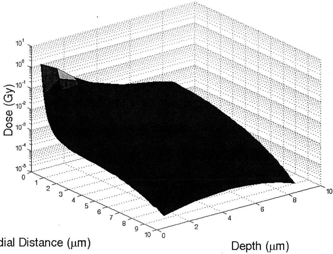
MCNP: 3-D Plot
