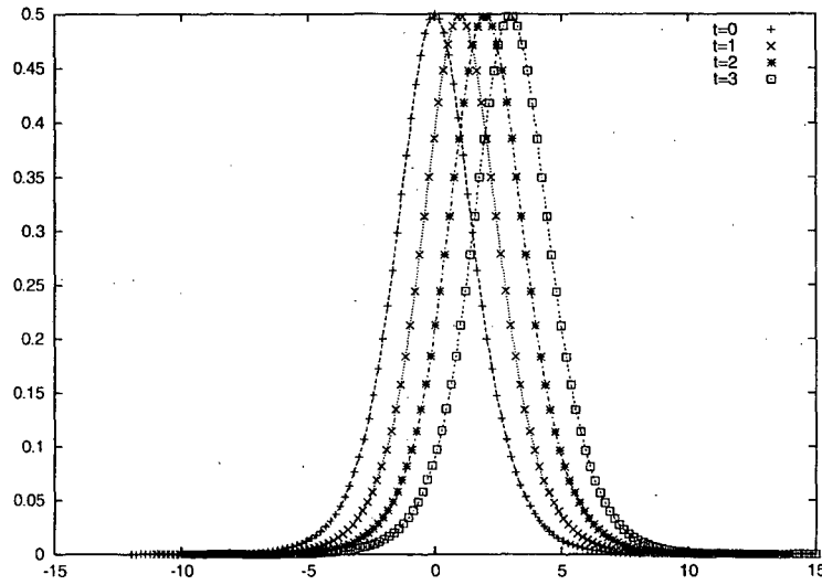
Figure 3.1: The solution of (2.1) with initial data (3.2) on [-12, 12] . N = 128 , \epsilon = \sqrt{h} . The points represent the location of the particles. The solid lines represent exact solution (3.3).
