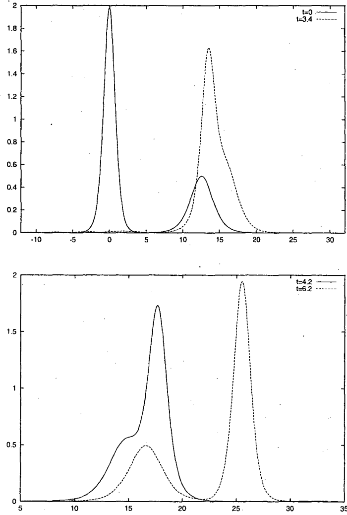
Figure 3.3: The solution of (2.1) with initial data (3.6) on [-3\pi, 10\pi] . N = 400 , \epsilon = \sqrt{h} .
