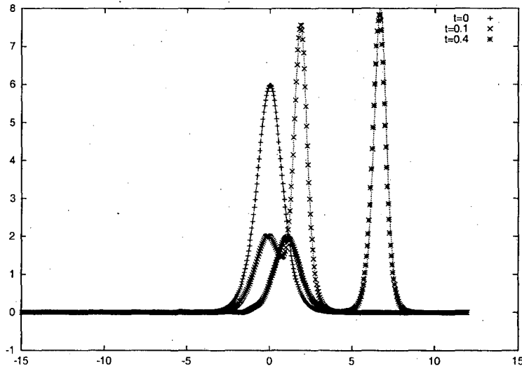
Figure 3.2: The solution of (2.1) with initial data (3.4) on [-15, 12] . N = 500 , \epsilon = \sqrt{h} . The points represent the location of the particles. The solid lines represent exact solution (3.5).
