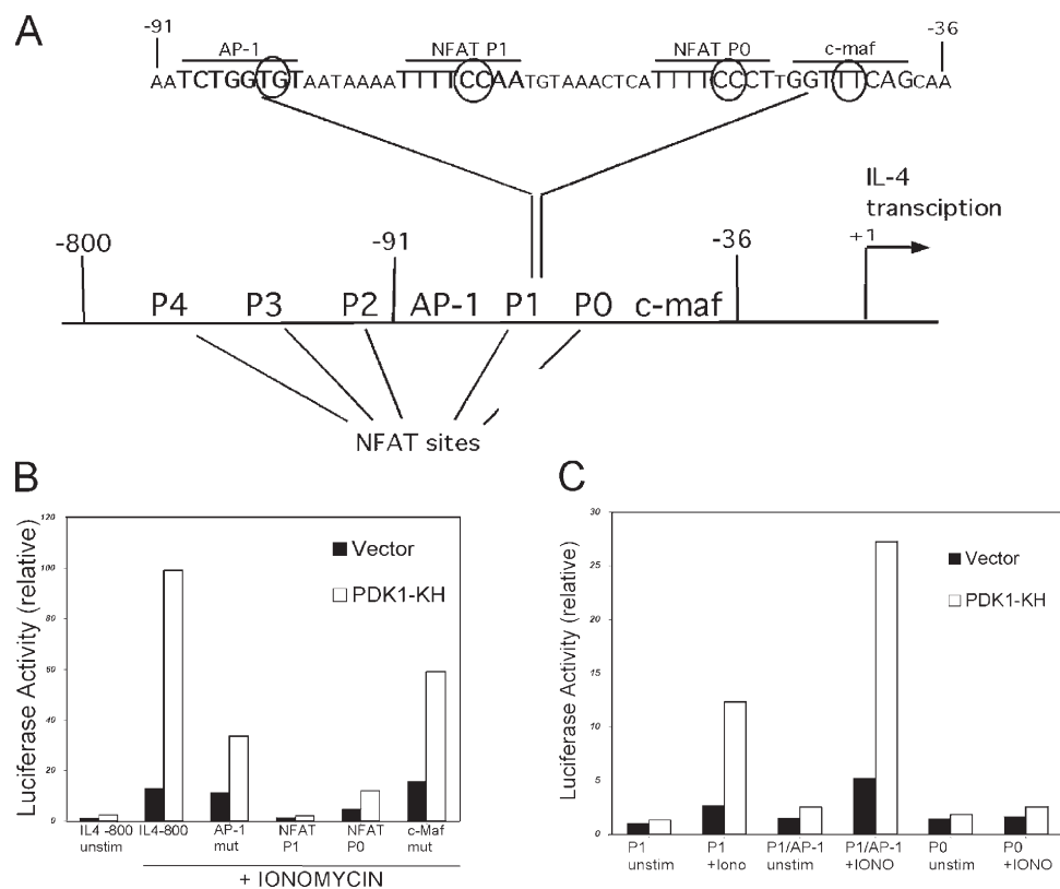
Figure 2. PDK1 targets the NFAT P1 site in the IL-4 promoter. (A) Schematic of the IL-4 promoter showing selected promoter elements and the sequence of the proximal promoter from -91 to -36 . The elements studied in this analysis are highlighted with larger letters with mutated nucleotides circled. (B) PDK1-KH activation of IL-4 requires the NFAT P1 site. PDK1-KH was coexpressed with wild type or mutant IL-4
